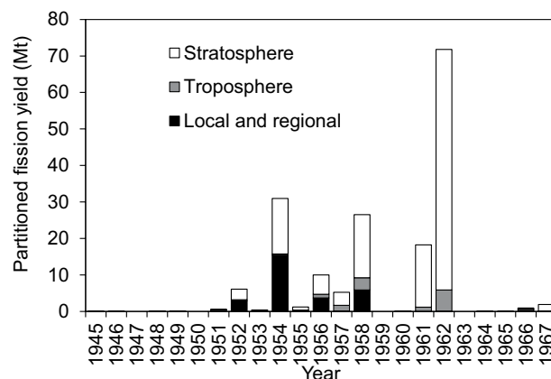
Figure 3. Annual fission yields injected into the stratosphere, troposphere, and local and regional atmospheric regions during 1945–1967 27 .
