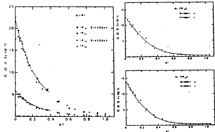
FIG.2. GOS vs the squared momentum transfer K^2 . The solid lines are obtained with the method of the least squares. The intercepts on longitudinal axis are the optical oscillator strengths.
