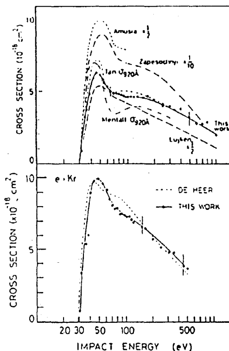
FIG.4. Absolute cross sections for the s-subshell ionization in Ar and Kr. Several results by other groups are also drawn for comparison.
