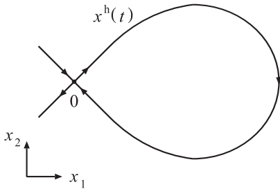
Figure 2: Homoclinic orbit x^h(t) on the x -plane
