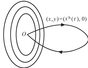
Figure 3: Periodic orbits near the origin
