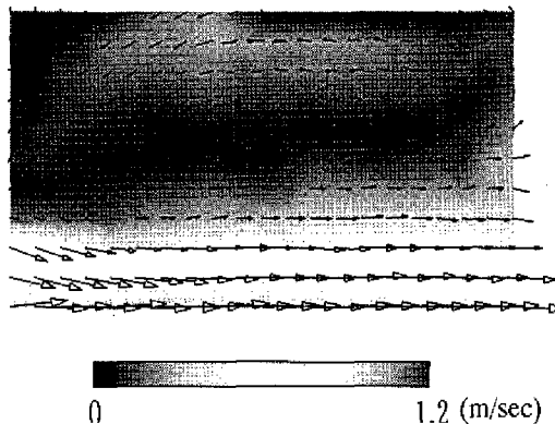
Fig. 8a Velocity vectors in the 2 nd embayment of the field, averaged over t = 0'00'' to 2'13''
