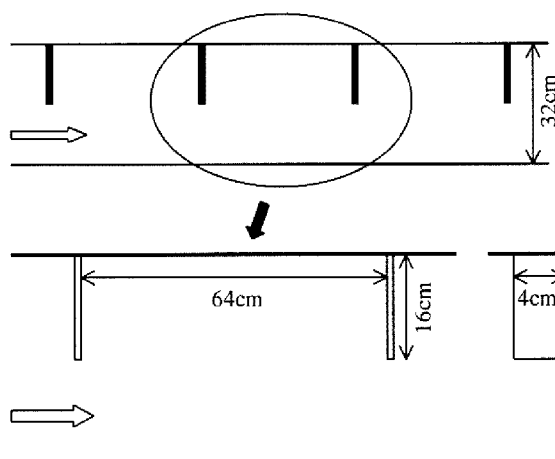
Fig. 11 Channel geometry for the laboratory experiments, top: the test section, bottom: a model embayment with spur dykes
