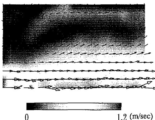
Fig. 8b Velocity vectors in the 2 nd embayment of the field, averaged over t = 3'30'' to 5'43''
