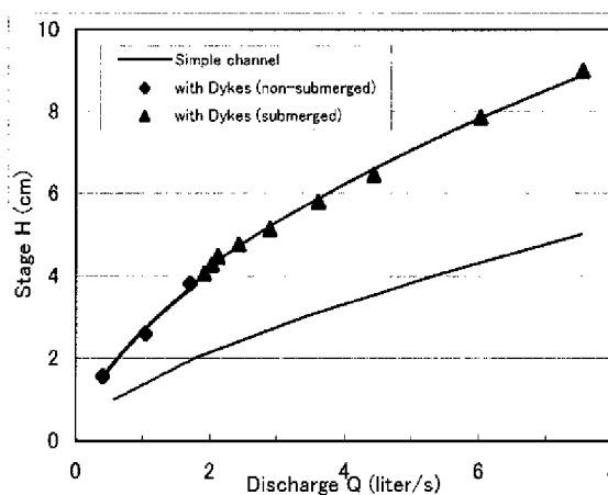
Fig. 13 Stage-discharge relationships for the simple rectangular channel with and without dykes
