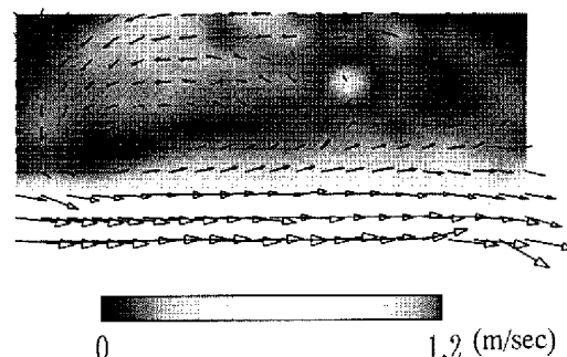
Fig. 10 Velocity vectors in the 3 rd embayment of the field, averaged over t = 3'30'' to 5'43''
