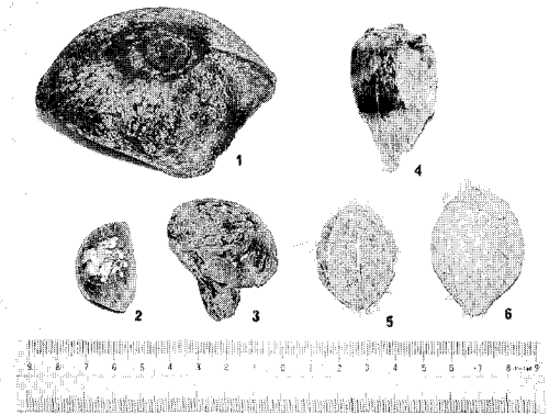
Fig. 1. Four species of tropical fruits that rarely stranded on the beach of Bansho-zaki at Shirahama, Wakayama Prefecture, Japan. 1: Xylocarpus granatum Koenig. 2, 3: X. sp. 4: Pandanus tectorius Parkinson. 5, 6: Terminalia catappa L.
