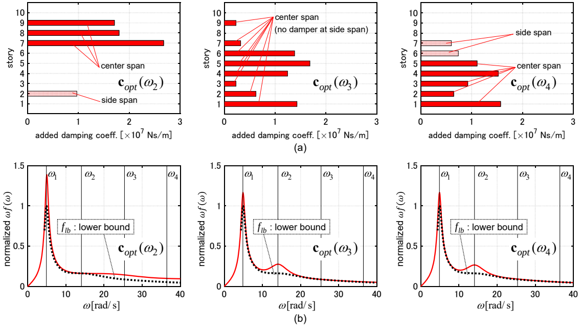
Fig. A3 Comparison of \mathbf{c}_{opt}(\omega_2) , \mathbf{c}_{opt}(\omega_3) , \mathbf{c}_{opt}(\omega_4) (moment resisting frame), (a) distributions of added damping coefficients, (b) normalized sum of transfer function amplitudes of interstory velocities.
