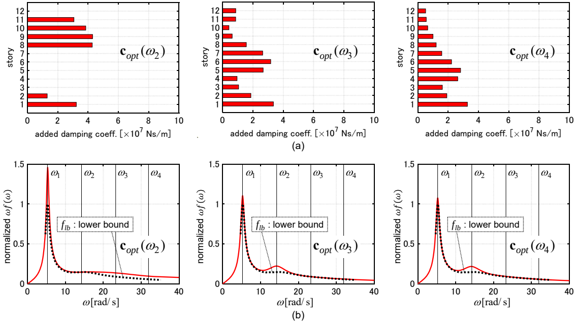
Fig. A1 Comparison of c_{opt}(\omega_2) , c_{opt}(\omega_3) , c_{opt}(\omega_4) (Model 1), (a) distributions of added damping coefficients, (b) normalized sum of transfer function amplitudes of interstory velocities.
