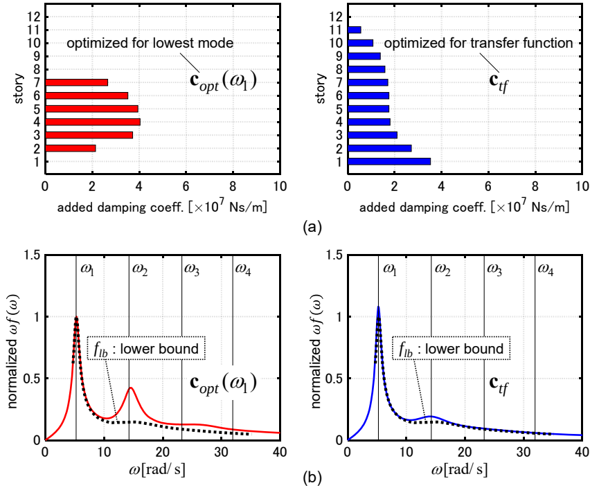
Fig. 5 Comparison of \mathbf{c}_{opt}(\omega_1) , \mathbf{c}_{tf} (Model 1), (a) distributions of added damping coefficients, (b) normalized sum of transfer function amplitudes of interstory velocities.
