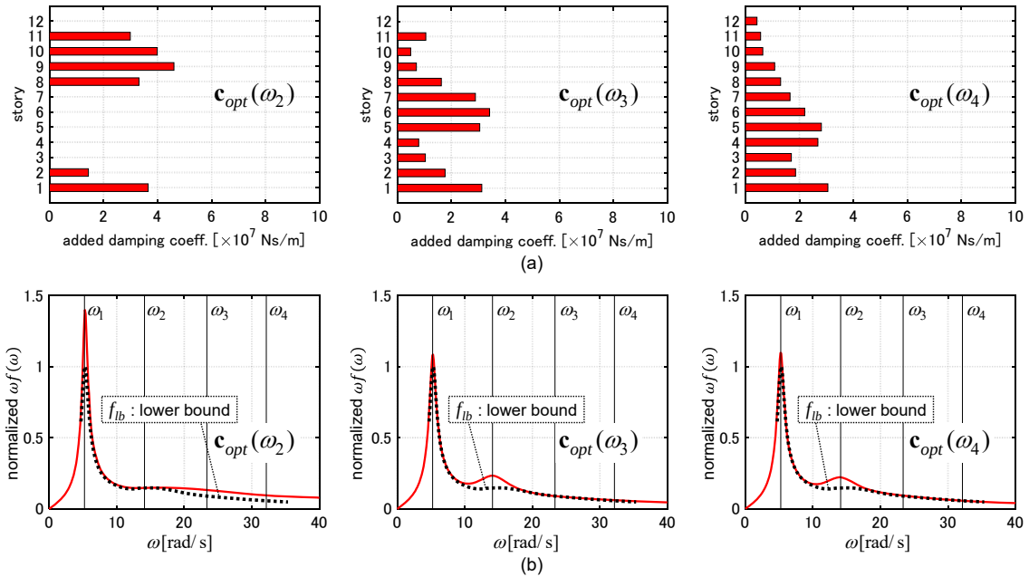
Fig. A2 Comparison of c_{opt}(\omega_2) , c_{opt}(\omega_3) , c_{opt}(\omega_4) (Model 2), (a) distributions of added damping coefficients, (b) normalized sum of transfer function amplitudes of interstory velocities.
