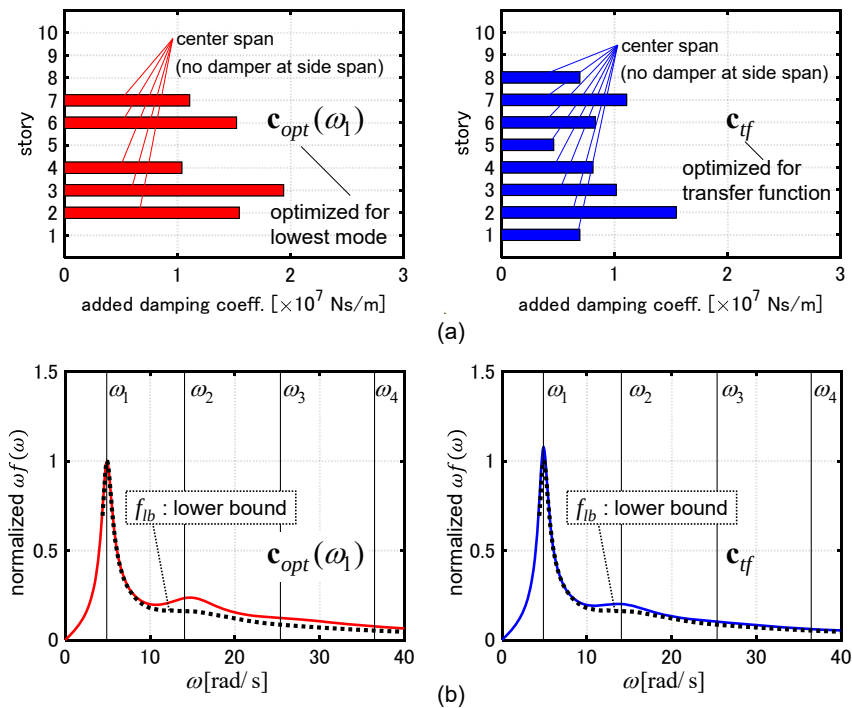
Fig. 11 Comparison of \mathbf{c}_{opt}(\omega_1), \mathbf{c}_{tf} (moment-resisting frame), (a) distributions of added damping coefficients, (b) normalized sum of transfer function amplitudes of interstory velocities.
