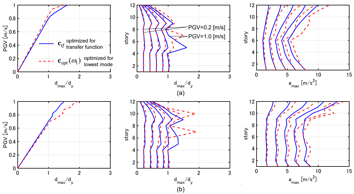
Fig. 9 IDA curves, distributions of maximum interstory drifts and distributions of maximum floor accelerations (Model 2), (a) El Centro NS component, (b) Taft EW component
