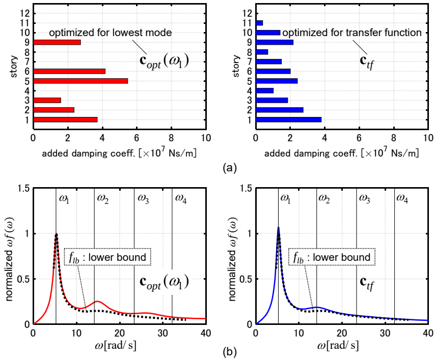
Fig. 6 Comparison of \mathbf{c}_{opt}(\omega_1) , \mathbf{c}_{tf} (Model 2), (a) distributions of added damping coefficients, (b) normalized sum of transfer function amplitudes of interstory velocities.
