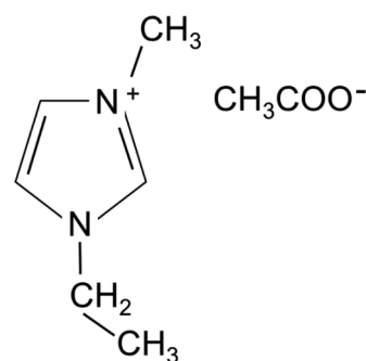
Fig. 1 Structural formula of the ionic liquid 1-ethyl-3-methylimidazolium acetate (abbreviated as EMI-CH 3 COO in the present paper)
