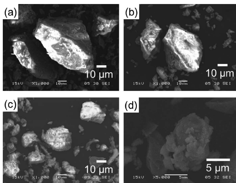
Fig. 2 Secondary electron images of various sizes of volcanic ash particles in sample A as received (without ionic liquid): (a) particle diameter 70 \mu m, (b) 50 \mu m, (c) 20 \mu m, and (d) 10 \mu m
