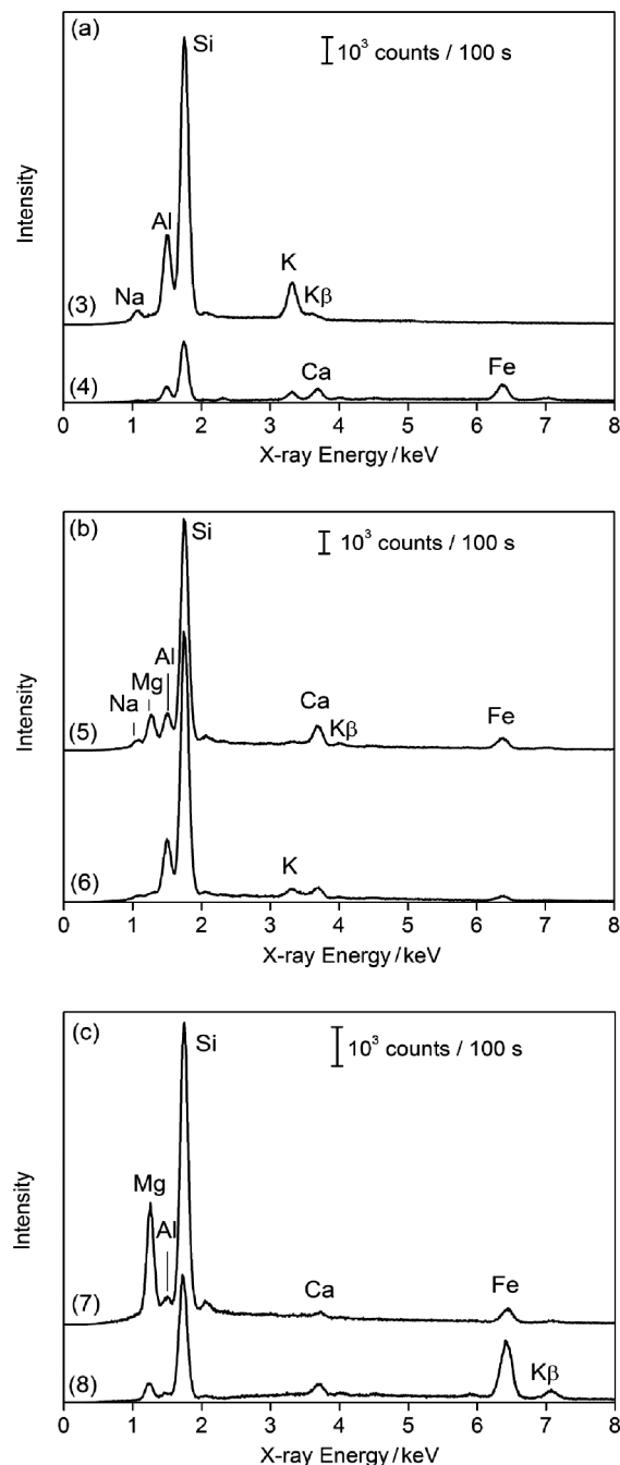
Fig. 6 SEM-EDX spectra of (a) sample C, (b) sample D, and (c) sample E, treated by the diluted ionic liquid Spectra (3)–(8) correspond to Fig. 5.
