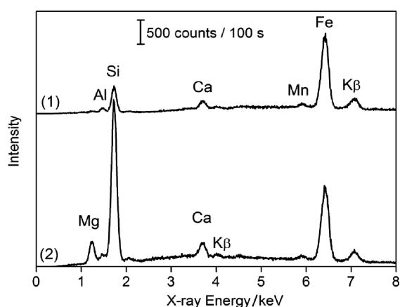
Fig. 4 SEM-EDX spectra of sample B treated by the ethanol diluted EMI-CH 3 COO (1 wt%)
