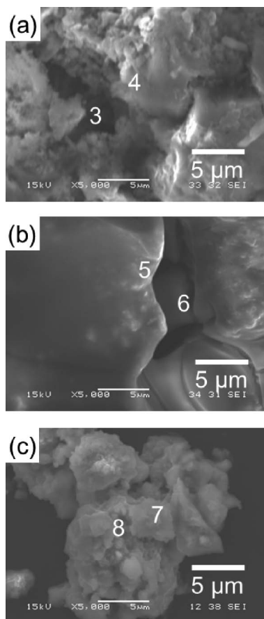
Fig. 5 Secondary electron images of (a) sample C, (b) sample D, and (c) sample E, treated by the ethanol diluted ionic liquid EMI-CH 3 COO (1 wt%) Positions 3–8 correspond to the spectra (3)–(8) in Fig. 6.
