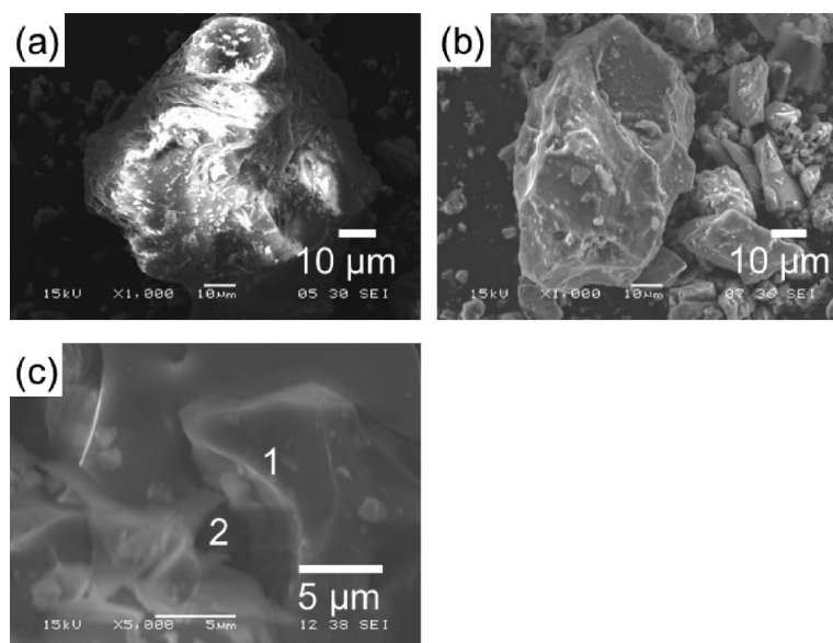
Fig. 3 Secondary electron images of volcanic aerosol particles in sample B, particle diameter of 70 \mu\text{m} : (a) as received, (b) with ethanol diluted EMI-CH 3 COO (1 wt%) treated, (c) enlarged image of (b), indicating the points 1 and 2 corresponding to the EDX spectra in Fig. 4
