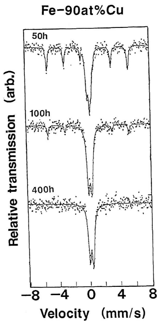
Fig.3.12 Changes of Mossbauer spectra of Fe-90at%Cu powder as a function of MA time.
