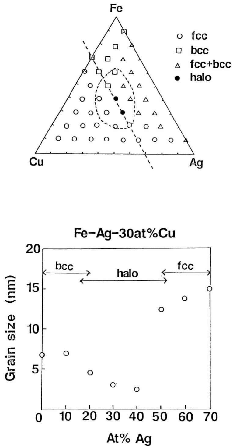
Fig.4.6 Grain size of MA 400h Fe-Ag-30at%Cu alloy evaluated from Scherrer formula.
