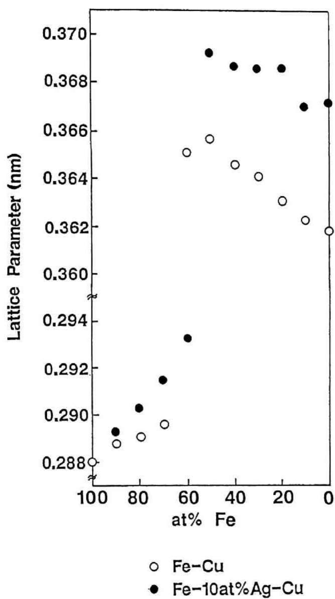
Fig.4.4 Lattice parameter of Fe-Cu and Fe-Ag-Cu alloy produced by MA 400h.
