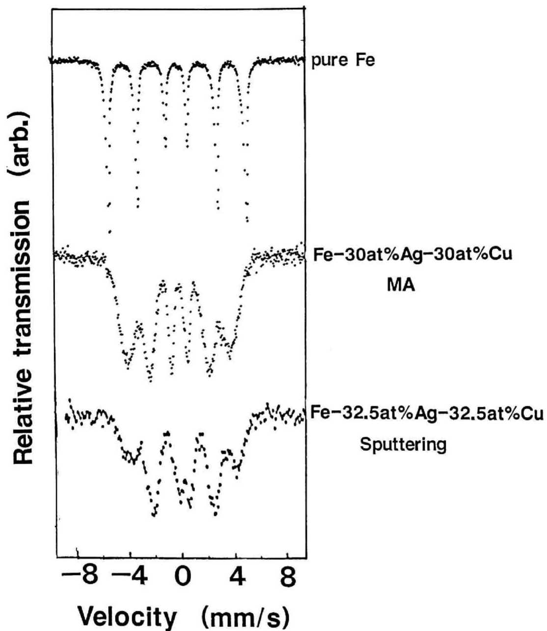
Fig.4.9 Mossbauer spectra of pur Fe, MA 400h Fe-30at%Ag-30at%Cu and sputter deposited Fe-32.5at%Ag-32.5at%Cu alloy.
