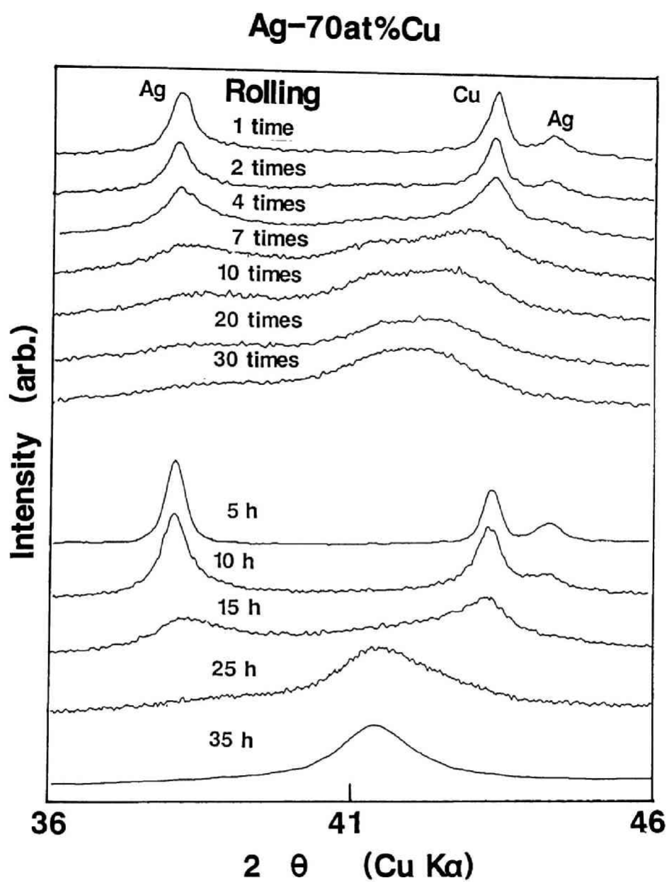
Fig.5.3 Changes of XRD patterns of Ag-70at%Cu powders as a function of rolling times and ball milling time.
