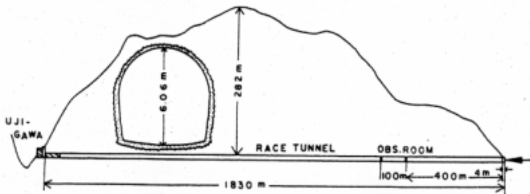
Fig. 1. Vertical section along the race tunnel.
