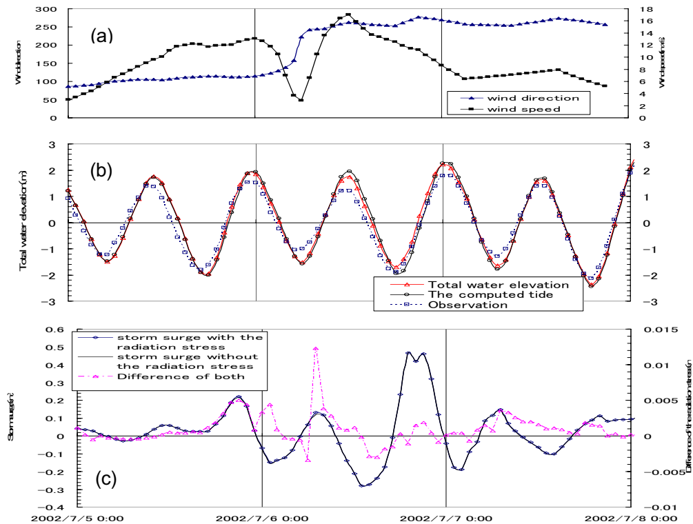
Figure 6. (a) the wind direction and speed; (b) the total water elevation of observation, the only computed tide and the computed total water elevation with the radiation stress; (c) the only storm surge considering the radiation stress, one without the radiation stress and difference of both at A (Yonggwang).
