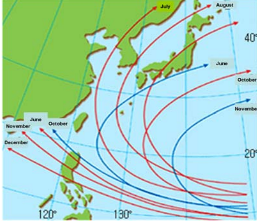
Figure 1. Typhoon tracks around the Korean Peninsula (from Korean Meteorological Administration)
