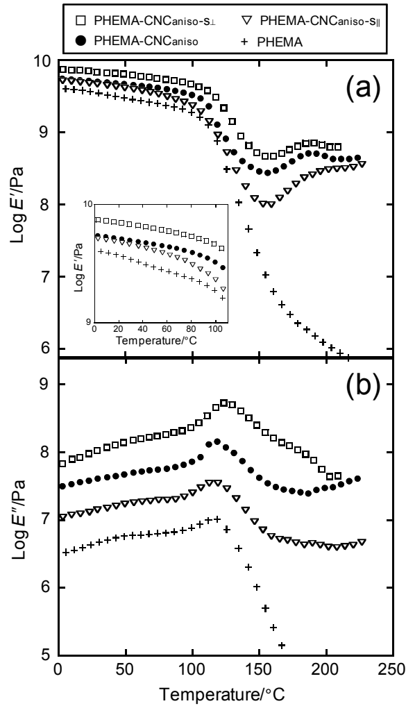
Figure 3-8. Temperature dependence of the storage modulus ( E' ) and loss modulus ( E'' ), measured in tension mode for film samples of PHEMA-CNC aniso -S, and PHEMA and PHEMA-CNC aniso references: (a) E' data for each sample, and an enlarged plot of the glass-state modulus E' (inset); (b) E'' data plotted by displaying by \sim 0.5 log unit in the ordinate. As to the PHEMA-CNC aniso -S composite, two rectangular strips distinguished from each other by notations \parallel and \perp (see Figure 3-9a) were used for the tension-mode DMA measurements.
