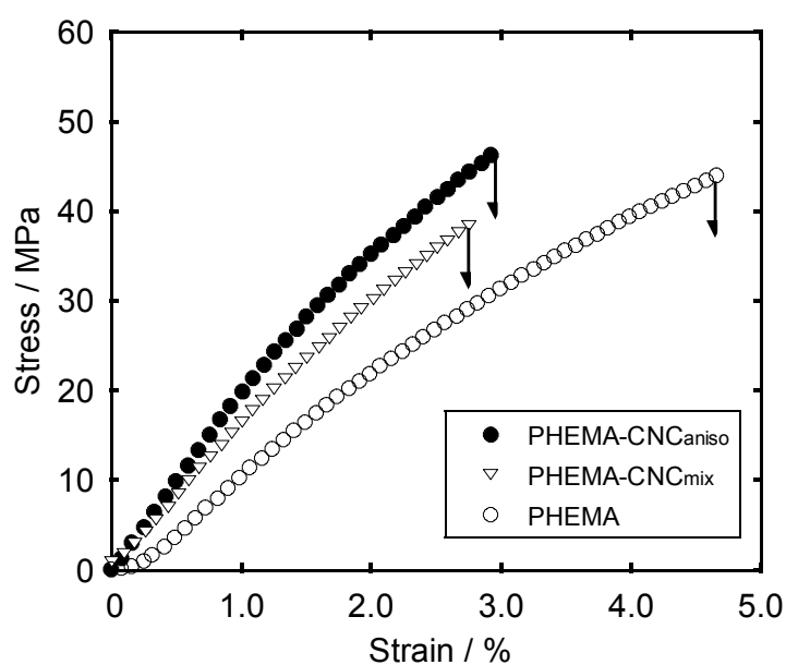
Figure 2-9. Examples of stress-strain curves measured for films of PHEMA, PHEMA-CNC aniso , and PHEMA-CNC mix .
