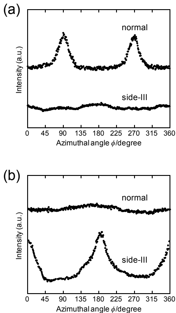
Figure 3-7. Azimuthal intensity profiles of the (200) diffraction of CNC: (a) data for PHEMA-CNC aniso-S ; (b) data for PHEMA-CNC aniso-T . These two composites are the same as those used in Figure 3-5. Intensity was scanned in the normal (upper) and side-III (bottom) views.
