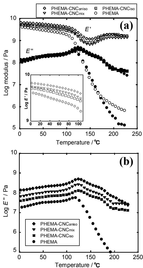
Figure 2-7. Temperature dependence of the storage modulus ( E' ) and loss modulus ( E'' ), measured for film samples of PHEMA and three PHEMA-CNC composites: (a) data in a set of E' and E'' for each sample, and an enlarged plot of the glass-state modulus E' (inset); (b) E'' data plotted by displacing by 0.25 log unit in the ordinate. See text for comparative discussion.
