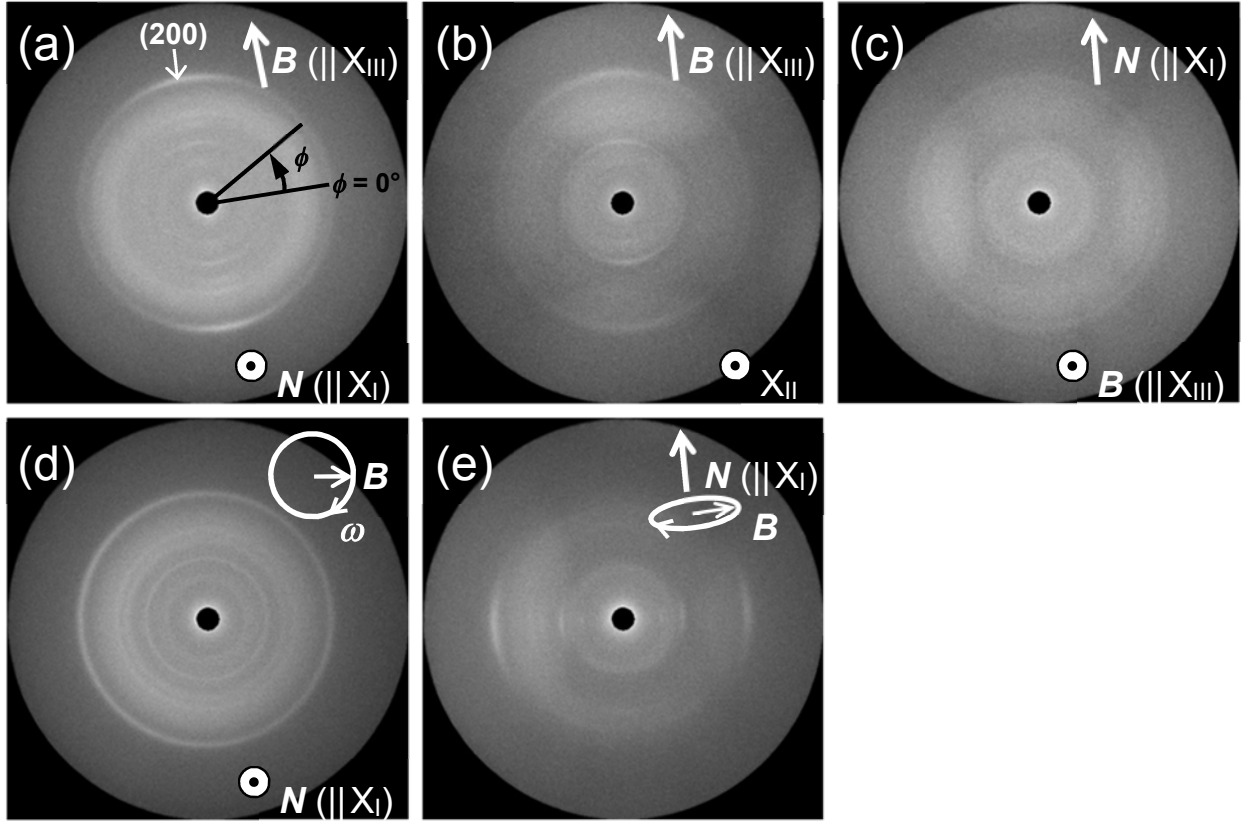
Figure 3-5. WAXD patterns of two polymer composites: (a) normal, (b) side-II, and (c) side-III views for PHEMA-CNC aniso-s ; (d) normal and (e) side-III views for PHEMA-CNC aniso-r . (See Figure 3-1c for definition of the views.)
