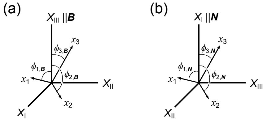
Figure 3-6. Pictorial representations specifying the orientation of a CNC frame O-x_1x_2x_3 of magnetic susceptibility with respect to the sample coordinate system O-X_I X_{II} X_{III} . The specification (a) is applicable to PHEMA-CNC aniso-s with the X_{III} -axis parallel to \mathbf{B} , and (b) refers to PHEMA-CNC aniso-r and -e with the X_I -axis parallel to \mathbf{N} .
