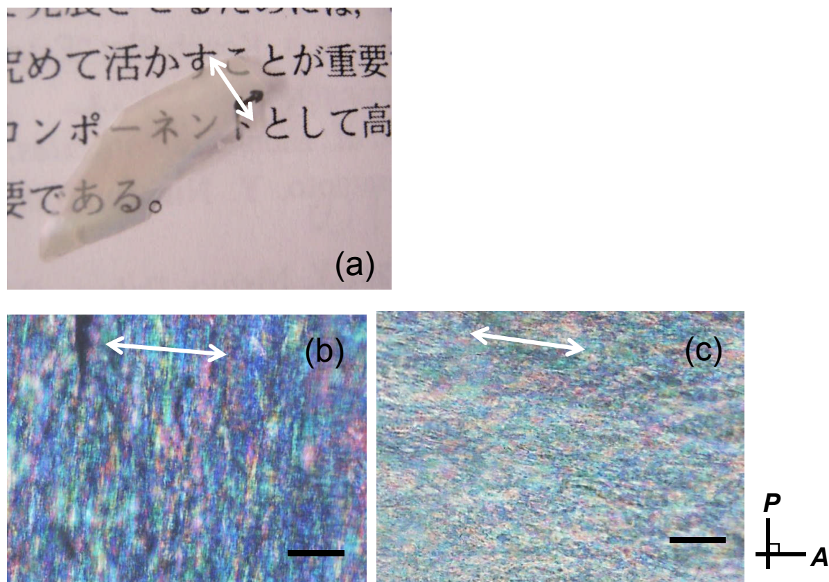
Figure 4-2. Visual appearance of a strip of CNC-2.0 (panel a), and polarized optical micrographs of CNC-2.0 (panel b) and CNC-6.7 (panel c) printed with a scale bar of 50 \mu\text{m} . White arrows indicate the shear direction (SD) of films.
