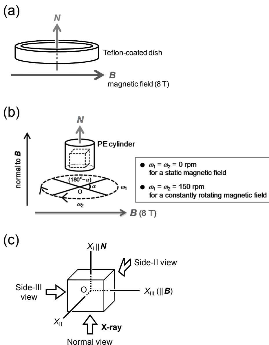
Figure 3-1. Schematic illustrations of the magnetic alignment systems using an 8 T field B : (a) application of a static magnetic field for preparing samples in film form; (b) applications of diverse magnetic fields for preparing samples in cylindrical form ( \omega_1 = \omega_2 = 0 for a static magnetic field and \omega_1 = \omega_2 = 150 rpm for a constantly rotating magnetic field); (c) setting up of a coordinate system O-X_I X_{II} X_{III} to each sample magnetically oriented, and definition of three views for WAXD measurements.
