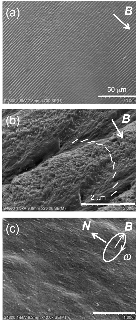
Figure 3-3. FE-SEM images of the fracture surfaces of polymer composites: (a) low-magnification data for PHEMA-CNC aniso-S ; (b) enlarged view of (a); (c) high-magnification data for PHEMA-CNC aniso-r .
