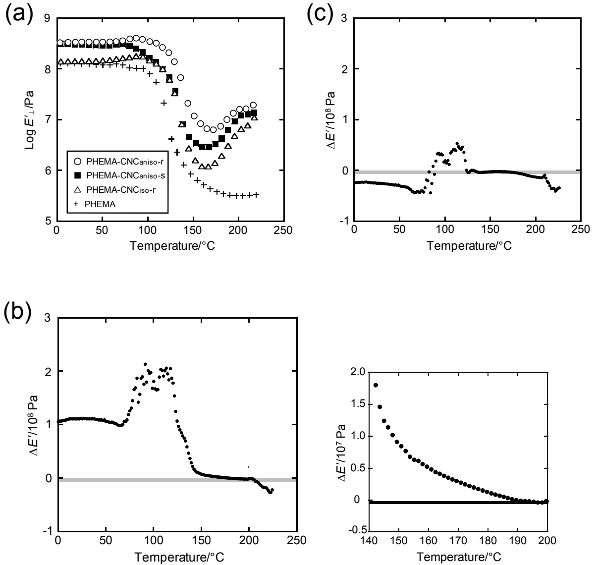
Figure 3-10. Temperature dependence of the modulus E'_{\perp} and differential \Delta E' ( = E'_{\perp} - E'_{\parallel} ), measured in compression mode for cuboid samples of PHEMA and various PHEMA-CNC composites: (a) E'_{\perp} data for PHEMA-CNC aniso-r , PHEMA-CNC iso-r , PHEMA-CNC aniso-s , and PHEMA (reference); (b) \Delta E' data for PHEMA-CNC aniso-r ; (c) \Delta E' data for PHEMA-CNC iso-r . Two compressive conditions for obtaining E'_{\perp} and E'_{\parallel} are depicted in Figure 3-9b.
