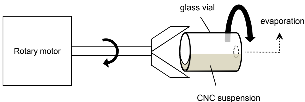
Figure 4-1. Schematic illustration of preparation of oriented CNC films from aqueous suspension by shearing under evaporation. The sample container (glass vial) was rotated at 700 rpm.
