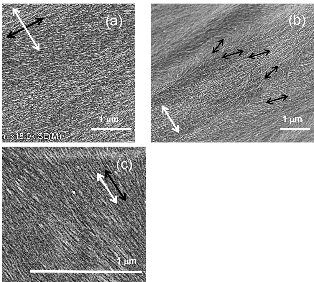
Figure 4-3. FE-SEM images of shear-deformed CNC films: (a) and (b) data for CNC-2.0; (c) data for CNC-6.7. White arrows indicate SD, and black arrows guide the alignment direction of fibrous entities (assimilation of CNCs) to the eye.
