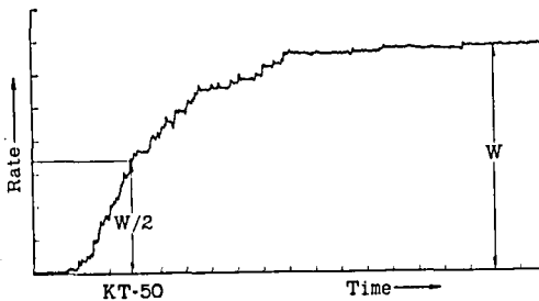
Fig. 2. The cumulative distribution curve of knocked-down houseflies.
