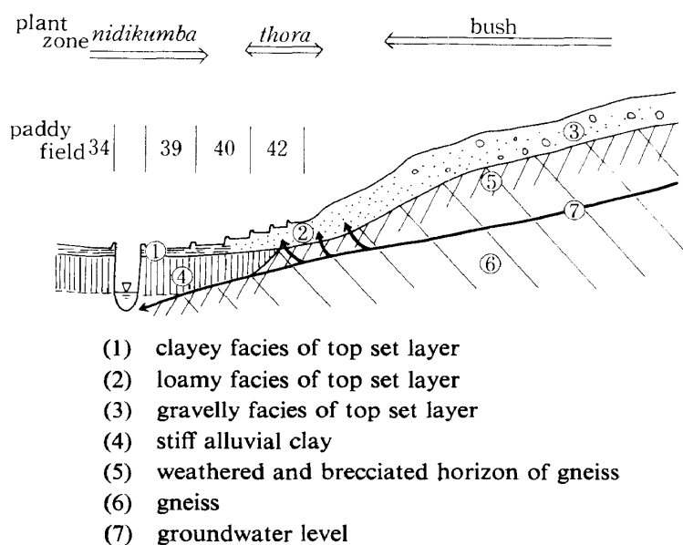
Fig. 8 A Cross-section through Puranawela , Akkarawela and Bushland, Showing Its Soil and Water Condition
