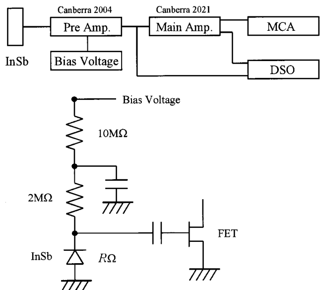
FIG. 4. Electronic circuit for alpha particle measurement (MCA: multi-channel analyzer, DSO: digital storage oscilloscope). Details of the input part of the preamplifier are shown.
