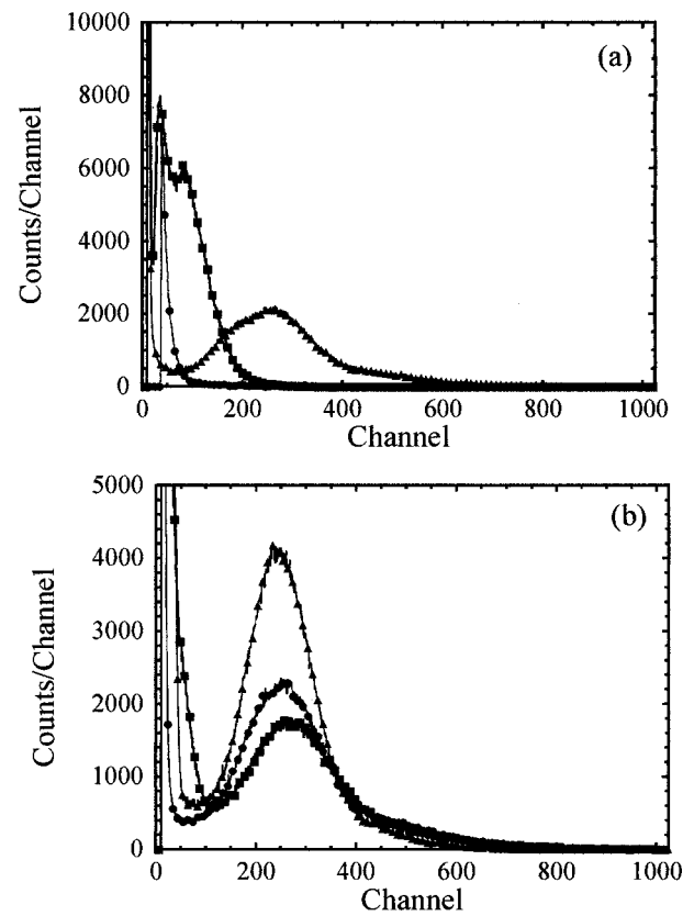
FIG. 6. Energy spectra of 241 Am alpha particles measured at operating temperature, shaping time, and applied bias voltage V_b of (a) 0.5 K, 0.25 μs, 1 V (solid circles), 3.5 K, 0.25 μs, 0 V (solid squares), and 3.5 K, 4 μs, 0 V (solid triangles); (b) 4.2 K, 4 μs, 0.5 V (solid circles), 4.2 K, 4 μs, 50 V (solid squares), and 4.2 K, 1 μs, 50 V (solid triangles), respectively. The voltage actually applied to the detector V_d is calculated by Eq. (1).
