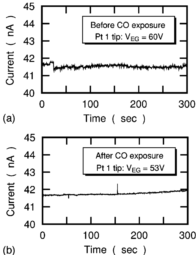
FIG. 2. Current fluctuation of the Pt emitter (a) before and (b) after exposure to CO gas.
