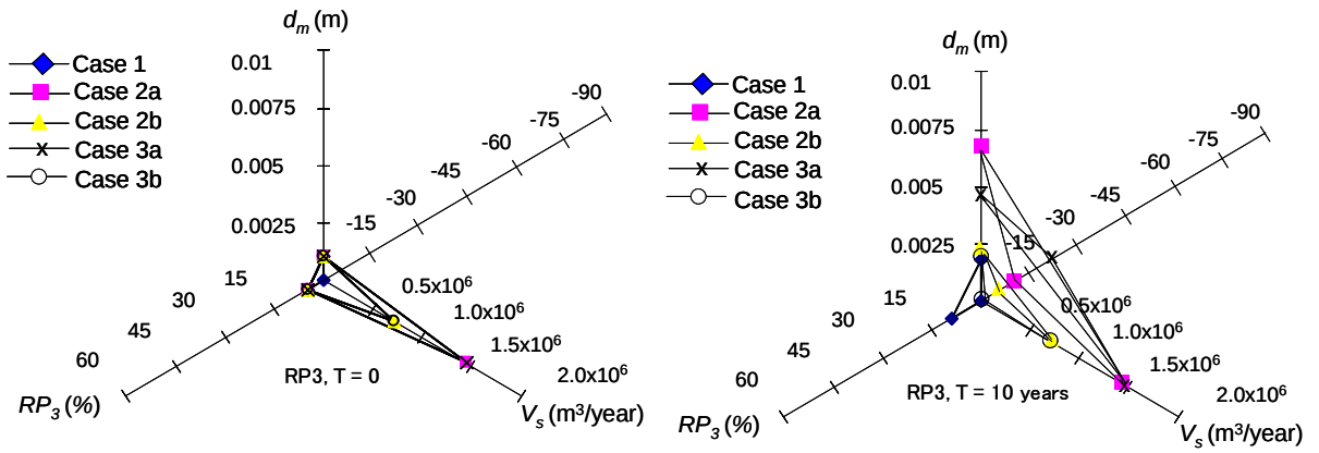
Fig. 4.36 Effect of sediment management on risk degree of bridge function ( RP_3 ), utilization, and environment at point 18 km from downstream boundary end
