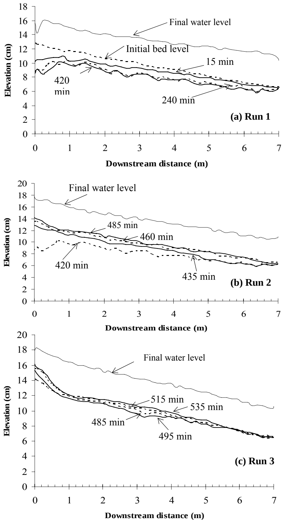
Fig. 4.62 Experiment results on bed surface and water surface in Run 1, Run 2, and Run 3.
