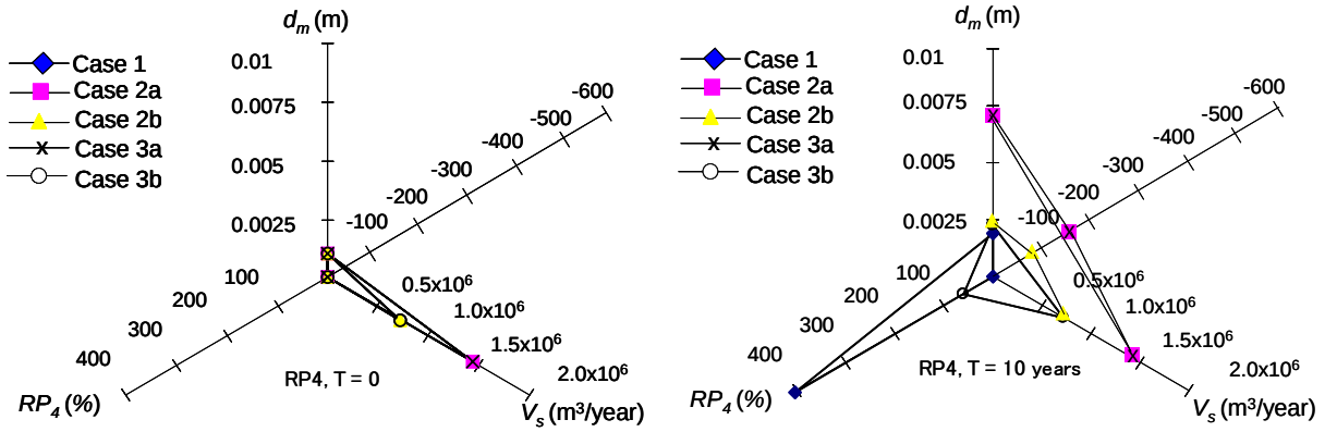
Fig. 4.27 Effect of sediment management on risk degree of sedimentation ( RP_4 ), utilization, and environment at point 30 km from downstream boundary end
