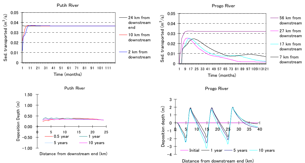
Fig. 3.55 Simulation result on sediment discharge and bed change in Case B-1 (without sabo works and no sand mining)
