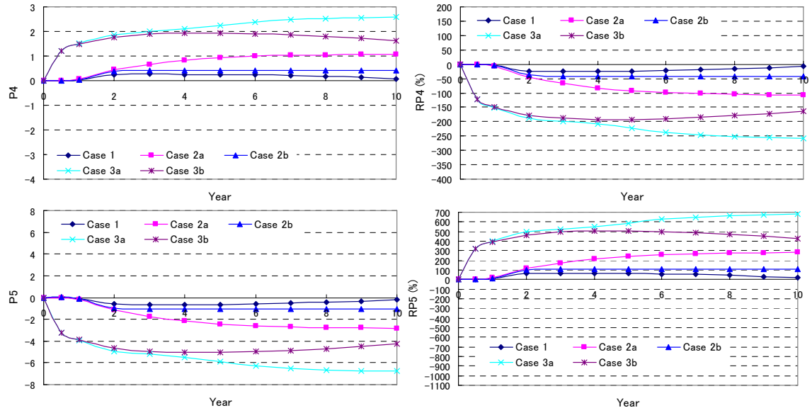
Fig 4.21 Effect of sediment management on the parameters P_4 , and P_5 ; and risk degree of the parameters P_4 , and P_5 at point 9 km from downstream boundary end
