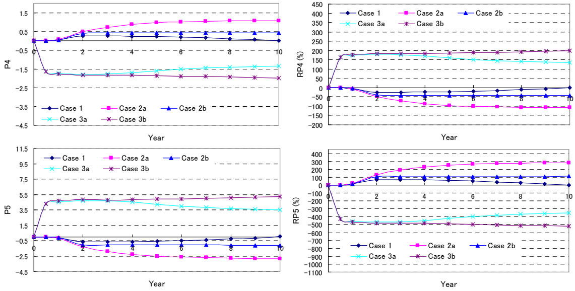
Fig 4.20 Effect of sediment management on the parameters P_4 , and P_5 ; and risk degree of the parameters P_4 , and P_5 at point 11 km from downstream boundary end
