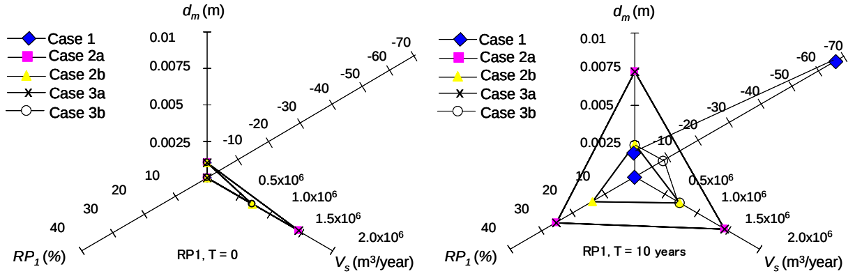
Fig. 4.24 Effect of sediment management on risk degree of bridge foundation function ( RP_1 ), utilization, and environment at point 30 km from downstream boundary end
