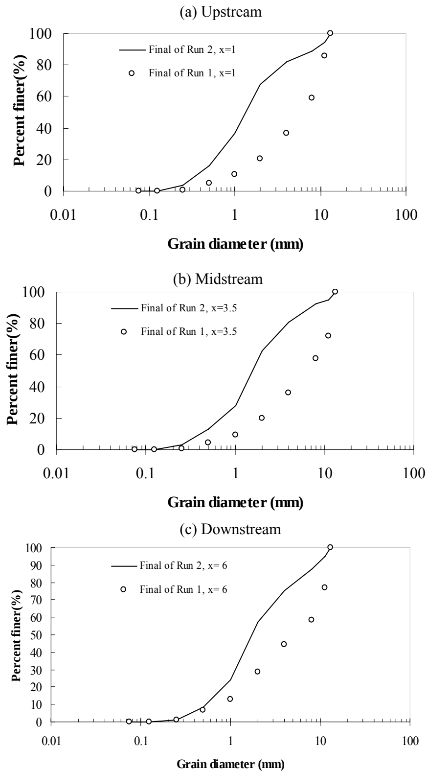
Fig. 4.64 Grain size distributions of surface bed material at the upstream ( x = 1 m), the midstream ( x = 3.5 m) and the downstream ( x = 6 m) after Run 2
