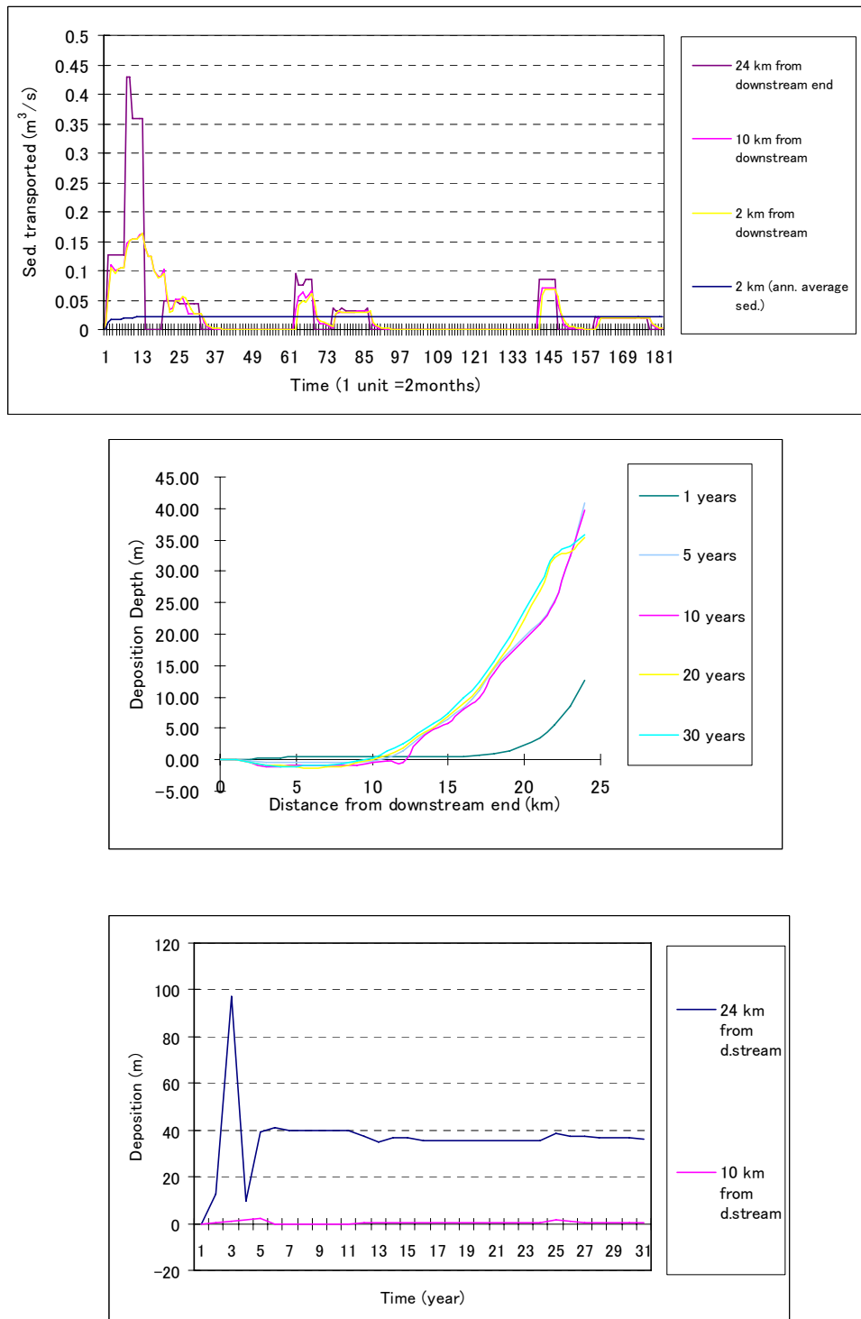
Fig. 3.57 Simulation result on sediment discharge and bed change with variation of sediment supply (without sabo works and sand mining (40%))
