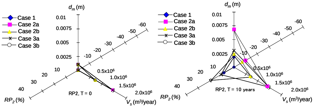
Fig. 4.30 Effect of sediment management on risk degree of pier bridge function ( RP_2 ), utilization, and environment at point 20 km from downstream boundary end
