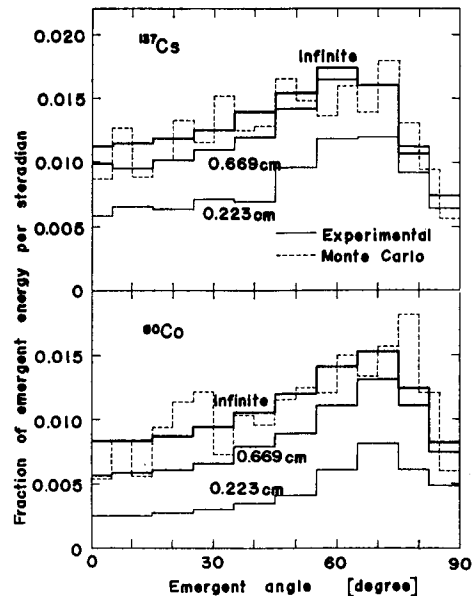
Fig. 5. Angular distribution of backscattered energies as a function of slab thickness. Asymptotic values \alpha_E(\theta, \infty) and Monte Carlo values 6) are also shown.
