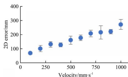
Figure 11 TDMA simulation result of 2D position error with different moving speeds
