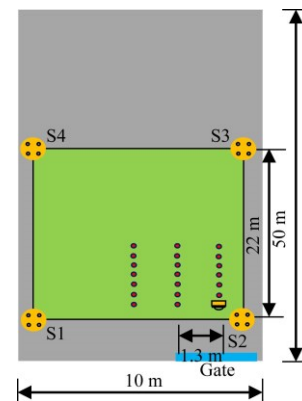
b. Experiment setup
