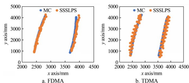
Figure 10 Dynamic movement of FDMA and TDMA
