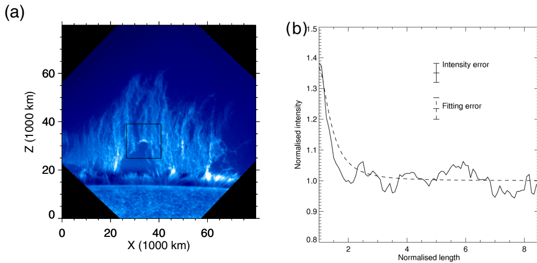
Figure: (a) A prominence with a plume (in the black box). The intensity increase at the head of the plume can be clearly seen. (b) The change of intensity with height at the head of the plume. Solid line shows the observed intensity and dashed line shows the result from the model.
