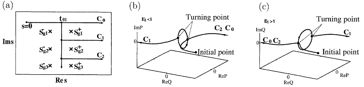
Figure 1: Singularities, integration paths and complex trajectories for the Eckart potential. (a) Singularities and representative integration paths on the lapse time plane. (b) Complex trajectories for E < 1 . (c) Complex trajectories for E > 1 .
