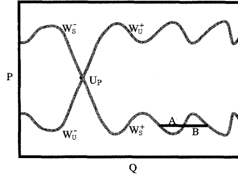
Figure 3: Schematic picture of the Poincaré map of the periodically perturbed system(eq.(5)). U_P denotes the unstable saddle. W_S^\pm and W_U^\pm indicate the stable and unstable manifolds of U_P , respectively.
