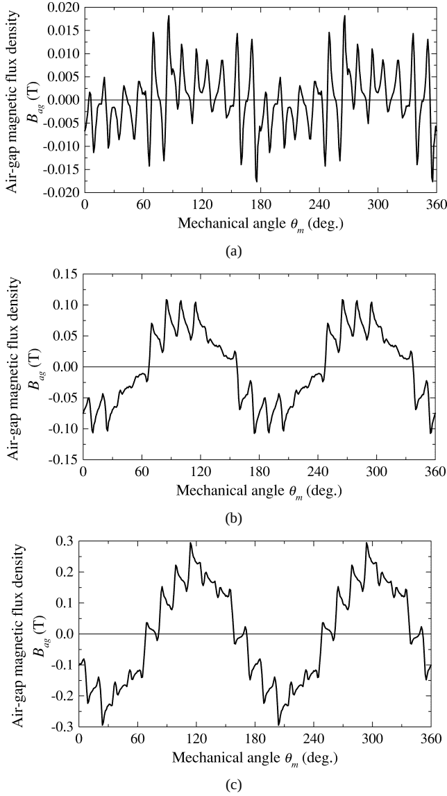
Fig. 3. Air-gap magnetic flux distribution at 77.3 K. (a) I_a = 1.0 A. (b) I_a = 2.0 A. (c) I_a = 4.0 A.
