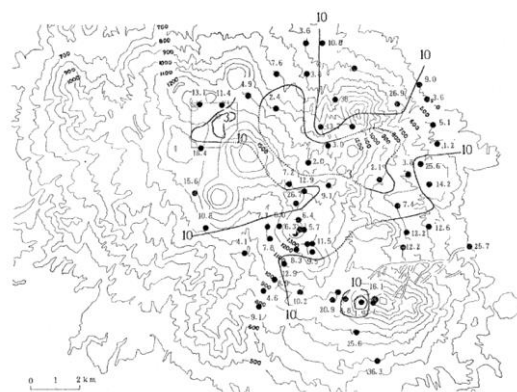
Fig. 6 Apparent resistivity distribution in Kirishima Volcanic Group by ELF-MT. Unit in \Omega \cdot \text{m} , 8Hz (Kagiyama, 1994).
