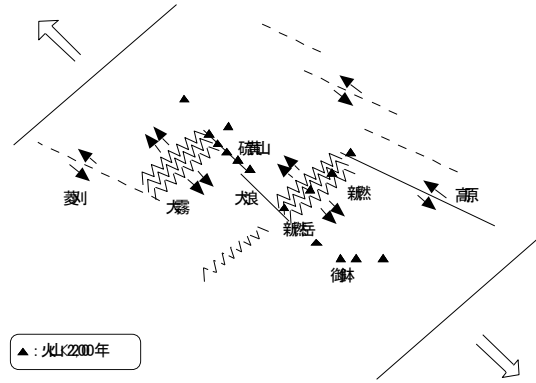
Fig. 9 Tectonic model around Kirishima Volcanic Group. The Kirishima area is subject to NW-SE extensional stress (Kagiyama, 1994).
