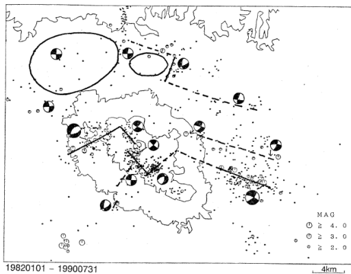
Fig. 8 Distribution of earthquakes and typical focal mechanism solutions around Kirishima (Kagiyama, 1992). Two ovals indicate epicentral areas of the earthquake swarms in 1968 and 1975 in the Kakuto Caldera.
