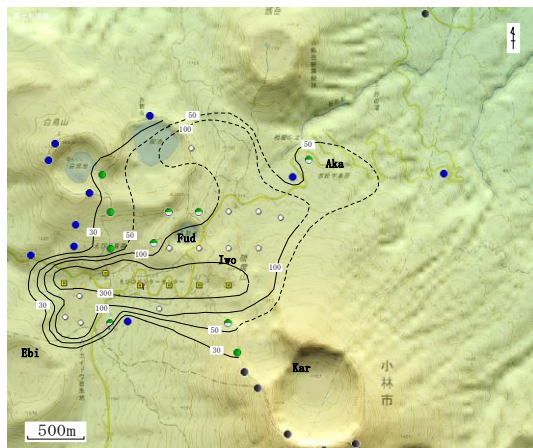
Fig. 4 Conductivity distribution in the surface layer
