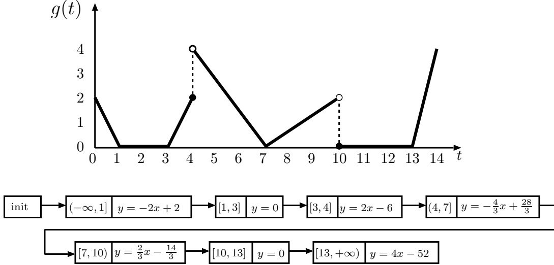
Figure 3.1: A function g and the linked list that represents g
