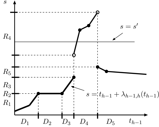
Figure 4.3: The relationship between the departure time t_{h-1} and the arriving time s = t_{h-1} + \lambda_{h-1,h}(t_{h-1})
