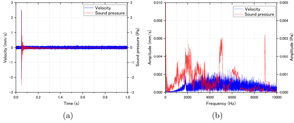
Figure 3: Vibration and sound in good concrete: (a) time history waveforms; (b) Fourier spectra of waveforms.
