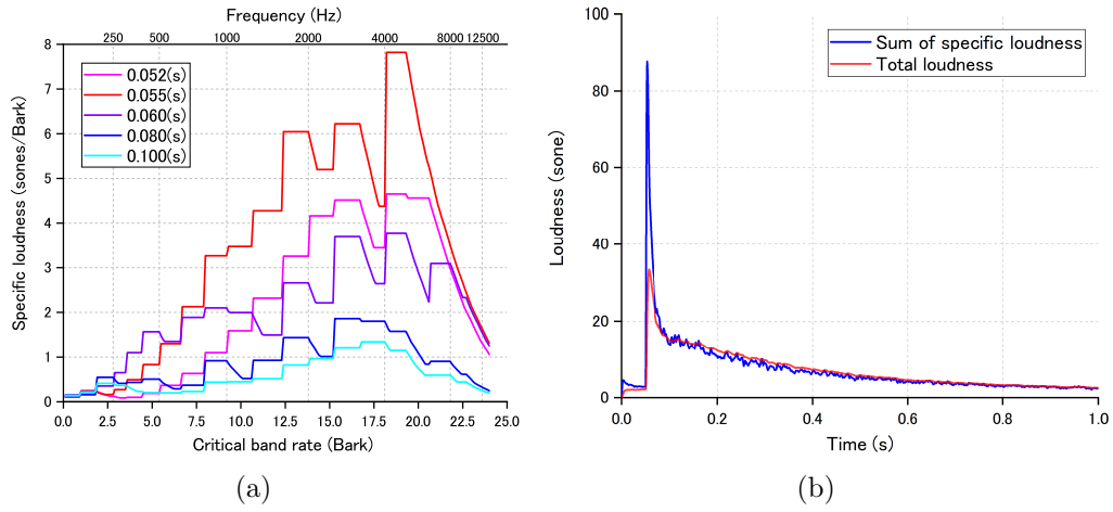
Figure 4: Loudness of hammering sound in good concrete: (a) specific loudness; (b) total loudness.
