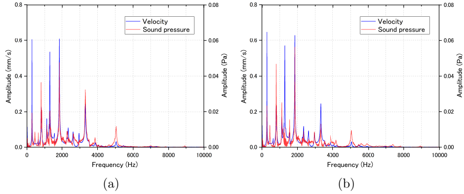
Figure 6: Fourier spectra of vibration and sound in specimen before cut. The sounds were measured at (a) position B and (b) position C.
