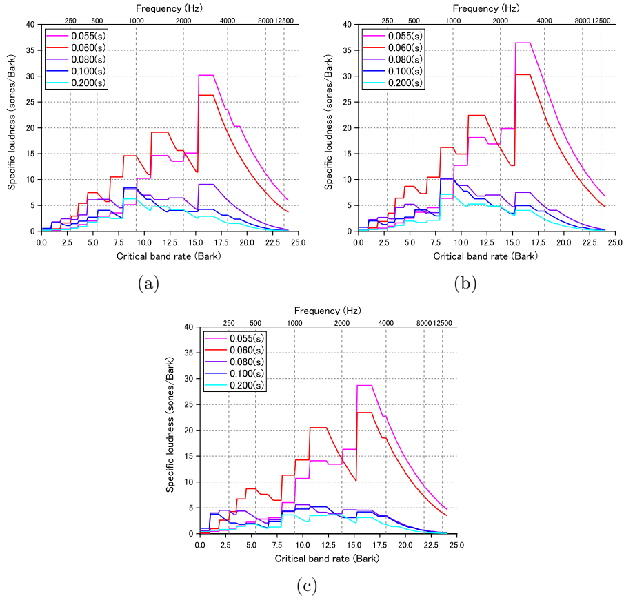
Figure 20: Specific loudness induced by impact hammer: (a) third impact; (b) fifth impact; (c) seventh impact. The cut length was 38 cm. The sounds were measured at position A.
