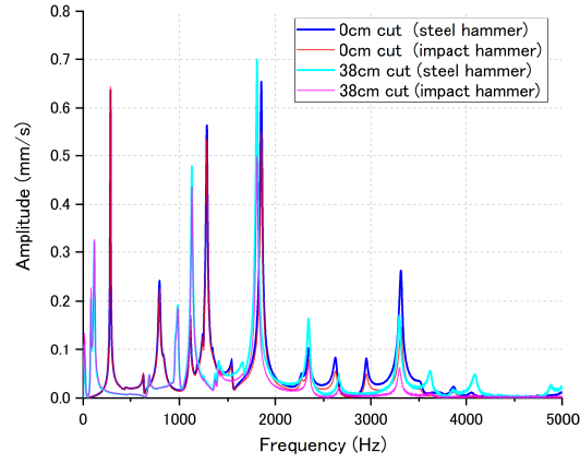
Figure 10: Comparison between Fourier spectra of vibration induced by steel hammer and Fourier spectra of vibration induced by impact hammer.
