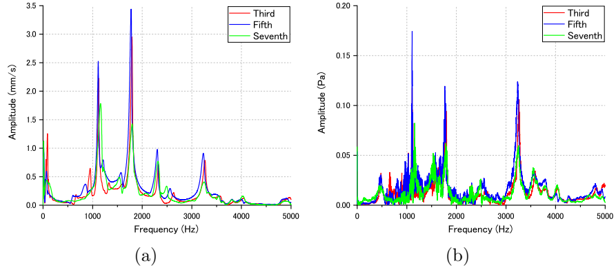
Figure 19: Fourier spectra of (a) vibration and (b) sound induced by impact hammer. The cut length was 38 cm. The sound was measured at position A.
