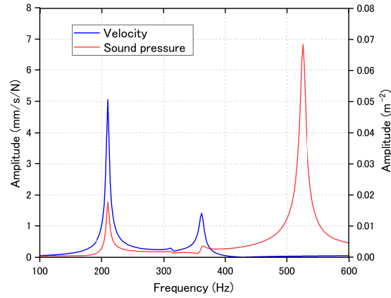
Figure 12: Frequency response functions obtained in specimen after cut of 30 cm, as obtained by numerical analysis. The sound was measured at position A.
