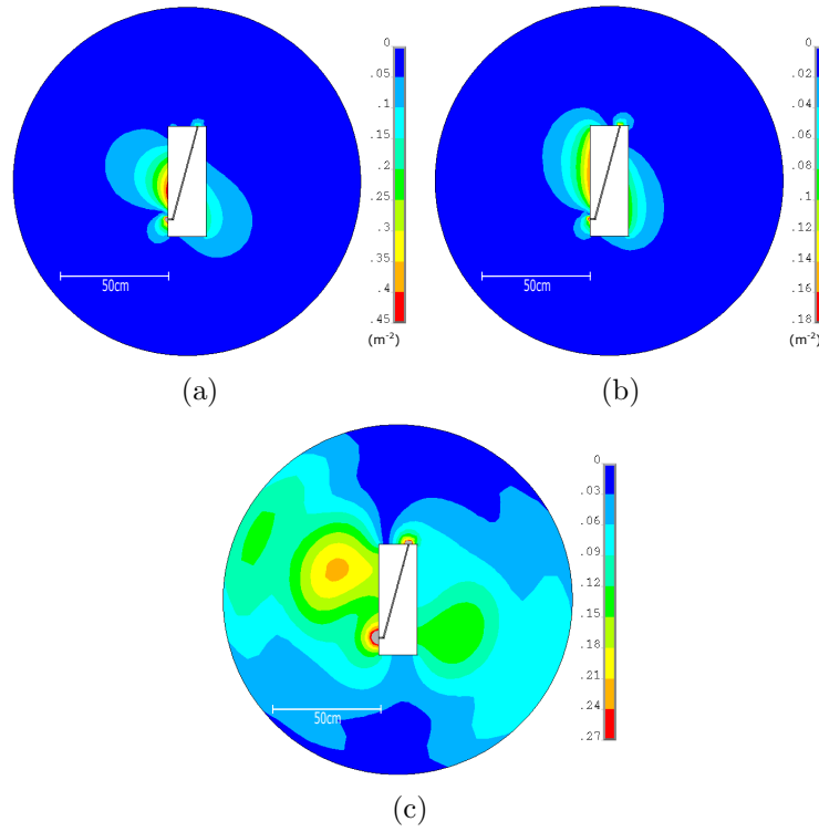
Figure 15: Spatial distribution of maximum sound pressure in specimen after cut of 30 cm on cross-section y = -10 (cm). The vibration frequency was (a) 210 Hz, (b) 362 Hz, and (c) 526 Hz.
