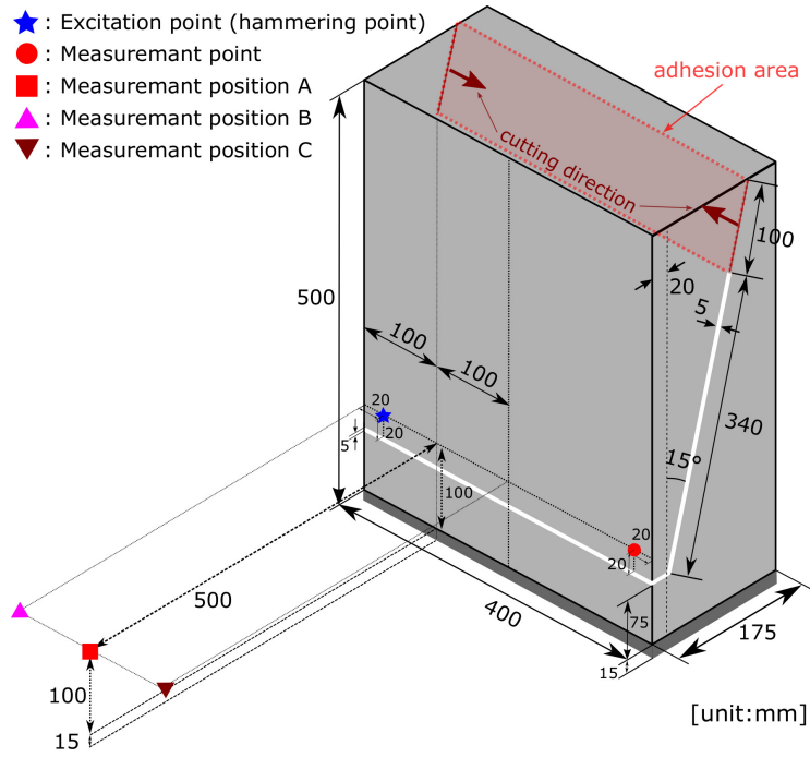
Figure 2: Dimensions of concrete specimen with vibration excitation and measurement points, and positions of sound pressure measurement.
