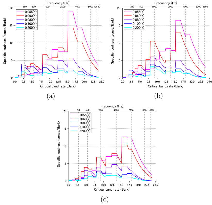
Figure 9: Change of specific loudness of sound with increase of cut length. The sound was measured at position A. The cut length was (a) 20 cm, (b) 30 cm, and (c) 38 cm.
