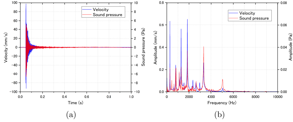
Figure 5: Vibration and sound in specimen before cut: (a) time history waveforms; (b) Fourier spectra of waveforms. The sound was measured at position A.
