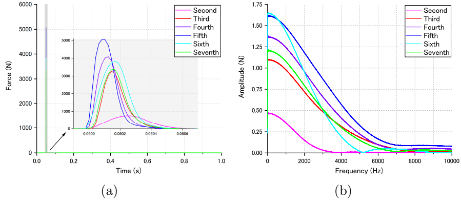
Figure 18: Force signals induced by impact hammer. The cut length was 38 cm: (a) time history waveforms; (b) Fourier spectra of these waveforms.
