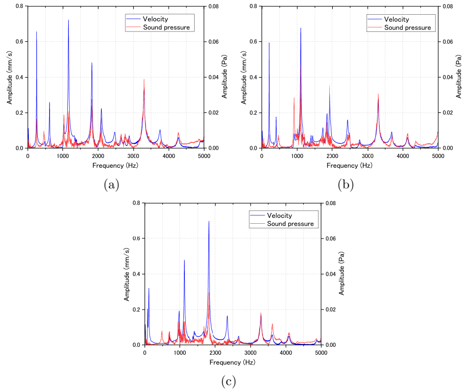
Figure 8: Change in Fourier spectra of vibration and sound with increase of cut length. The sound was measured at position A. The cut length was (a) 20 cm, (b) 30 cm, and (c) 38 cm.
