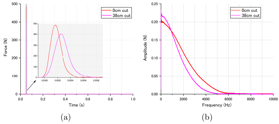
Figure 11: Force signals induced by impact hammer: (a) time history waveforms; (b) Fourier spectra of these waveforms.
