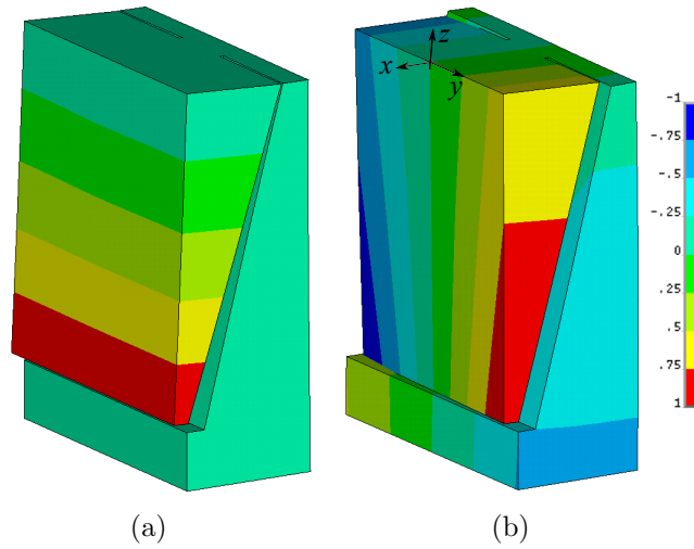
Figure 13: Deformation in x -direction of low-order vibration modes in specimen after cut of 30 cm. The natural frequency was (a) 210 Hz and (b) 362 Hz.
