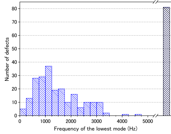
Figure 1: Distribution of lowest mode frequency in defect area rated as \beta in unreinforced concrete sections of tunnels.
