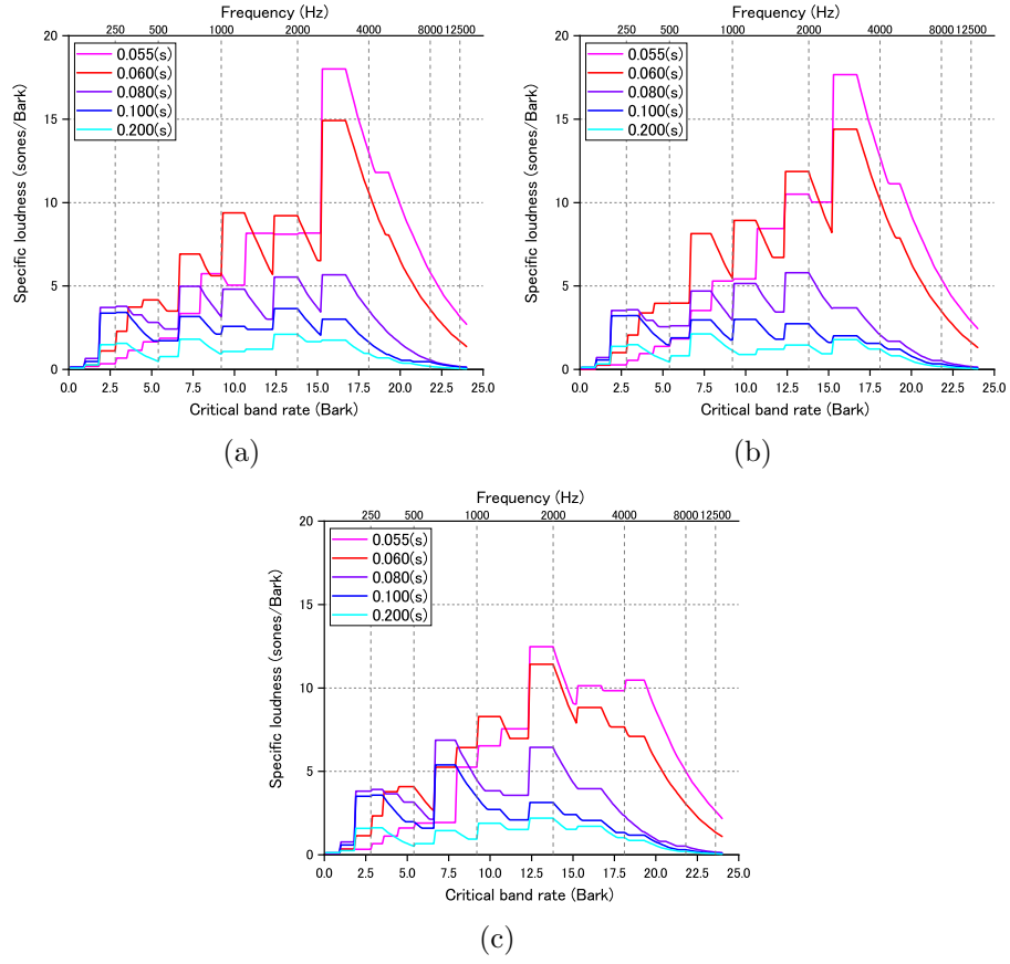
Figure 7: Specific loudness of hammering sound in specimen before cut. The sounds were measured at (a) position A, (b) position B, and (c) position C.
