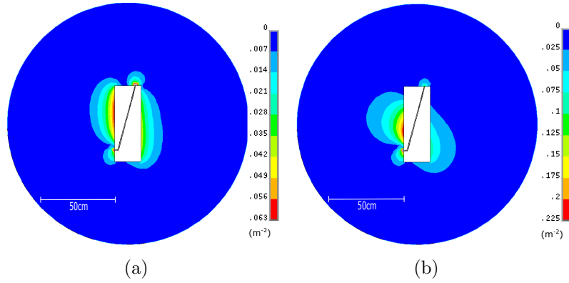
Figure 17: Spatial distribution of maximum sound pressure on cross-section y = -10 (cm) in specimen after cut of 38 cm. The vibration frequency was (a) 98 Hz and (b) 152 Hz.
