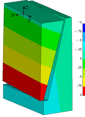
Figure 14: Deformation in z -direction of low-order vibration modes in specimen after cut of 30 cm. The natural frequency was 314 Hz.
