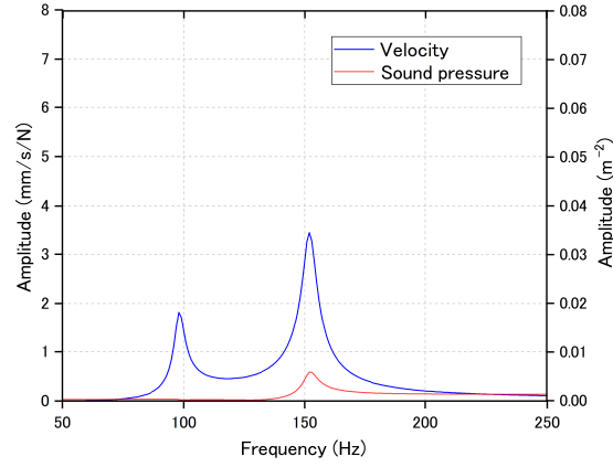
Figure 16: Frequency response functions in specimen after cut of 38 cm, as obtained by numerical analysis. The sound was measured at position A.
