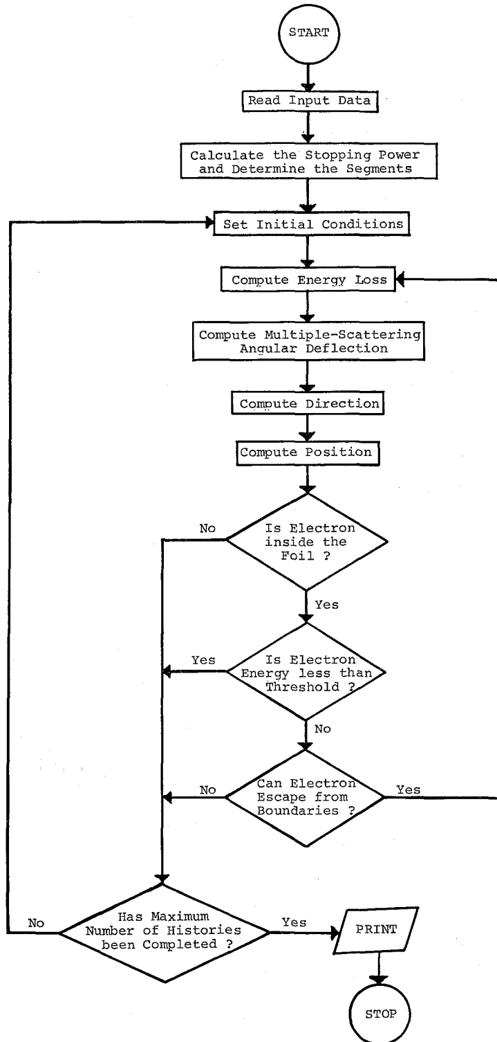
Fig. 1. Schematic flow diagram of the program.
