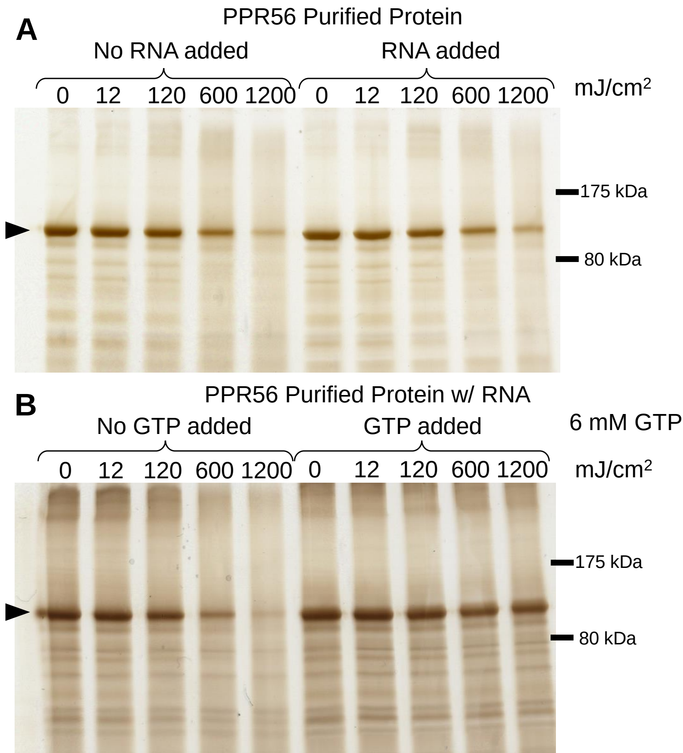
Figure 21: GTP stabilizes the PPR56 monomer when exposed to crosslinking UV radiation
