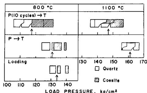
Fig. 9. Results of runs on the quartz-coesite transition. Arrows show the transition points. For other explanation, see text.
