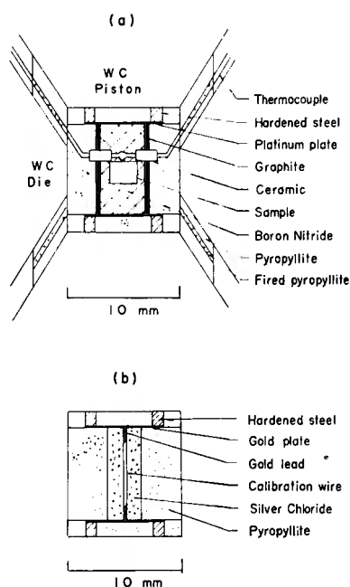
Fig. 1. The internal configuration of gasket and specimen cell. (a) The design used for the quenching method at high temperatures. (b) The cell used for the calibration at room temperature.
