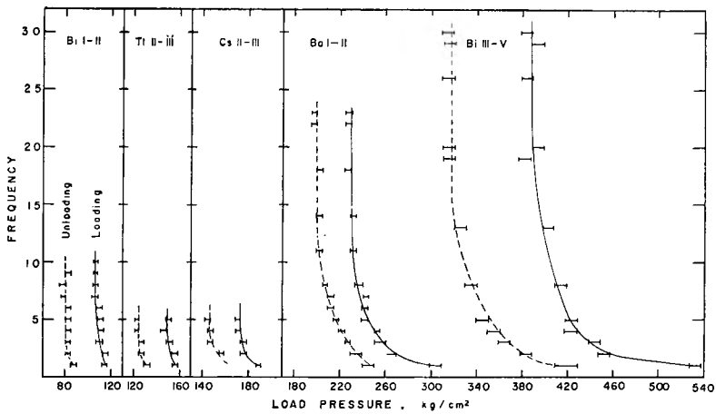
Fig. 7. Typical examples of the effect of repeated loading.
