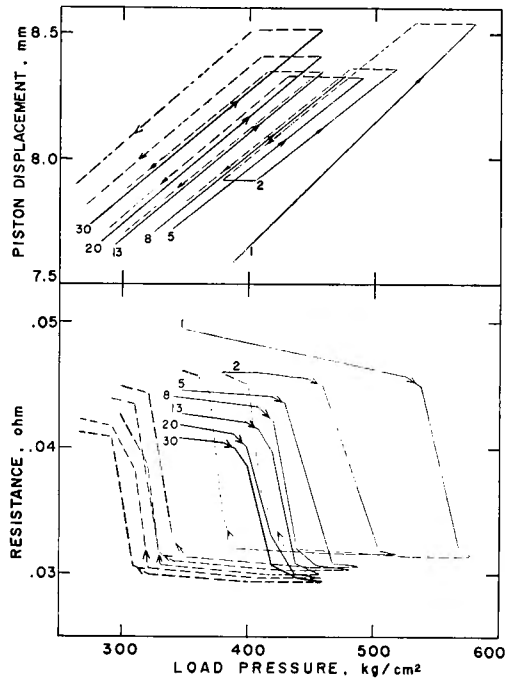
Fig. 6. Typical cycles through the Bi III-V transition (lower) and the corresponding ones of piston travel (upper). The solid lines are on loading and the dashed on unloading. The transition points are illustrated by arrows. The number is the frequency of repetition of the cycles on loading and unloading.
