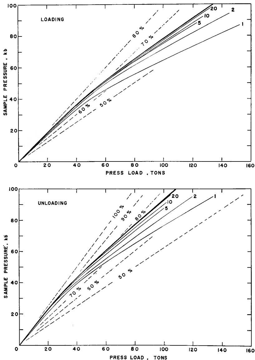
Fig. 8. Pressure calibration curves for every frequency of repetition of the girde apparatus on loading and unloading. The thick curves are from the convergent values. The dashed lines are the efficiencies. The number is the frequency of repetition.
