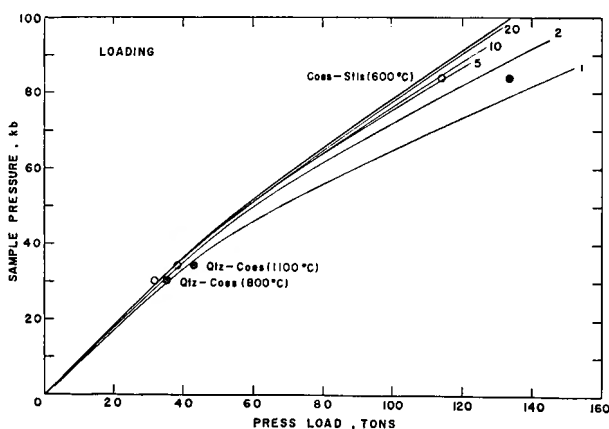
Fig. 10. Comparison of the pressure at high temperatures with the calibration curves at room temperature on loading runs. Solid circles are of the first loading. Open circles are of the loading after the ten time repetition in the quartz-coesite transitions and after the twenty time repetition in the coesite-stishovite transition.
