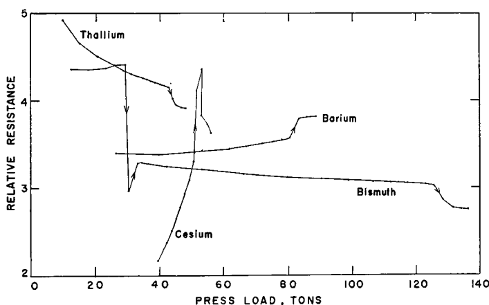
Fig. 3. Typical resistance changes of bismuth, thallium, cesium and barium observed in the cell shown in Fig. 1b.
