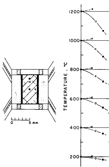
Fig. 2. The temperature gradients in the graphite furnace. The left side shows the distribution of the measured points in the cell; the solid circle: the center of the furnace, the open and the double circles: 2 mm and 3 mm distant from the center in the direction of length, respectively, the cross: 1.5 mm distant from the center in the direction of radius. The right side shows the temperatures at the corresponding points as a function of distance from the center.
