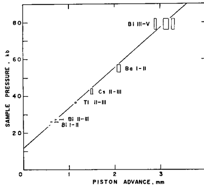
Fig. 5. Relationship between sample pressure and piston advance of the girdle apparatus for the first loading. Piston advance is normalized at the value for 13.43 ton of press load.
