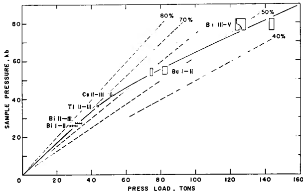
Fig. 4. Pressure calibration curve of the girdle apparatus for the first loading. The dashed lines are the efficiencies of the generated pressure to applied load.
