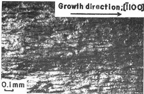
Fig. 8. Corrugations of a 99.9% Zn single crystal grown in [1100] at the rate of 1.7 mm/min.
