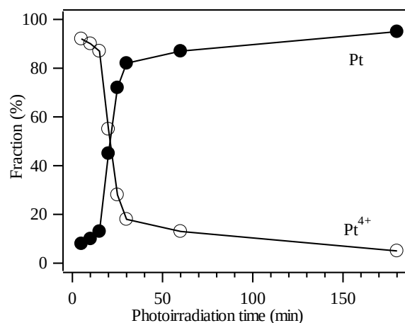
Figure 4. Dependence of the fractions of Pt metal and \text{Pt}^{4+} ions on the photoirradiation time.
