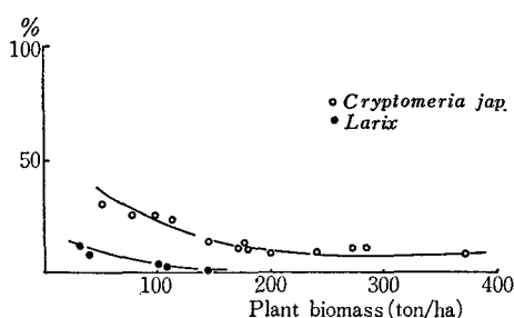
Fig. 7-a. Proportion of leaves to total plant biomass
