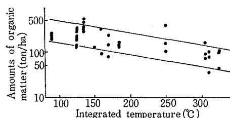
Fig. 2. Relationship between the amount of organic matter in soils and the integrated temperature
