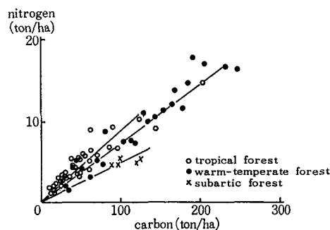
Fig. 8. Amounts of carbon and of nitrogen in soils.
