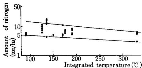
Fig. 9. Relationship between the amount of nitrogen in forest ecosystems and the integrated temperature
