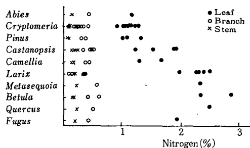
Fig. 6. The nitrogen concentration of leaves, branches and stems of different tree species
