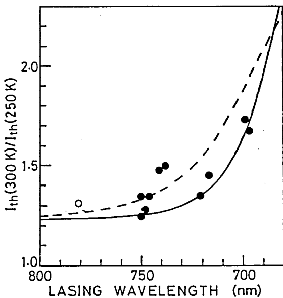
Fig.13 Experimental and calculated threshold-temperature coefficient I_{th}(300\text{ K})/I_{th}(250\text{ K}) for the low temperature range as a function of the lasing wavelength. Notations are the same as those indicated in Fig.12.
