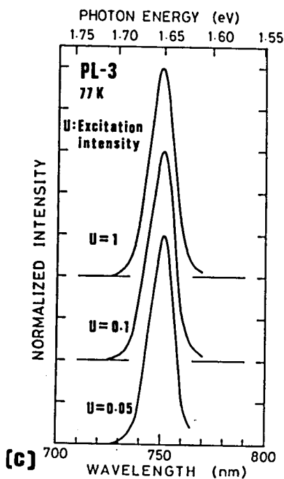
Fig.19 Variation in photoluminescence spectra with excitation intensity of (a) PL-1, (b) PL-2, and (c) PL-3 at 77 K. Measurements were carried out by excitation with 632.8-nm light from a He-Ne laser.
