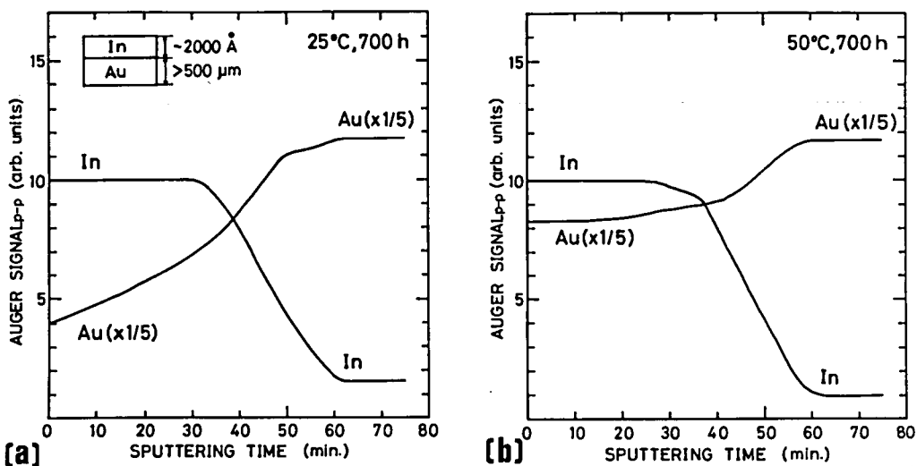
Fig.18 Auger depth composition profiles of samples for simulation after storage for 700 h at (a) 25 and (b) 50°C. Auger signals were corrected for Auger sensitivity and differential sputtering of Ar ion etching used in measurements.
