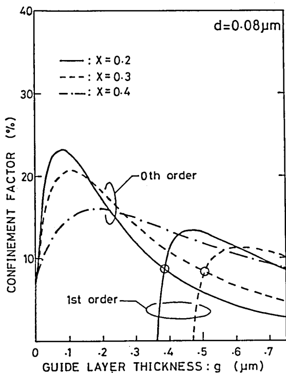
Fig.2 Confinement factor \Gamma as a function of guide layer thickness. The AlAs mole fraction in the guide layer is given by x . Open circles indicate that \Gamma is equal for the fundamental and the first order transverse modes and thus give g_0 .
