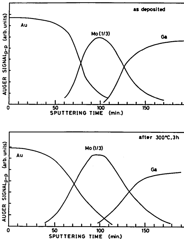
Fig.15 Auger depth composition profiles of Mo( \sim 500 Å)/Au( \sim 1000 Å) evaporated on GaAs (a) before and (b) after a heat treatment at 300°C for 3 h.
