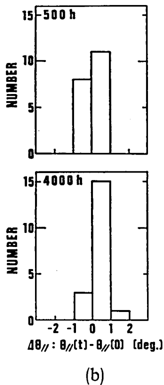
Fig.17 (a) A typical example of lateral far-field patterns measured before (0 h) and after the agings of 500 and 4000 h under 5 mW/facet at 50°C. (b) Relative change of full-width at half-power (FWHP) of far-field pattern from 0 h after aging.
