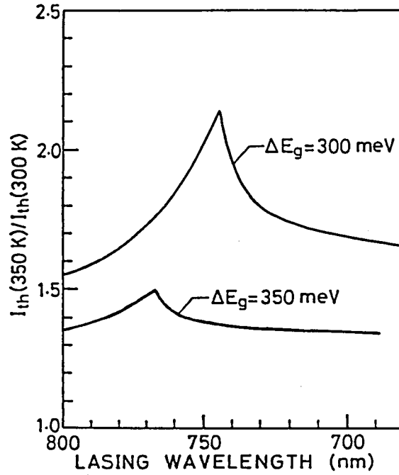
Fig.15 Calculated I_{th}(350\text{ K})/I_{th}(300\text{ K}) for \Delta E_g = \text{constant} and \eta_i = \text{constant} . In the case of \Delta E_g = 350\text{ meV} , the shortest wavelength is limited by the AlAs mole fraction of unity in the cladding layer.
