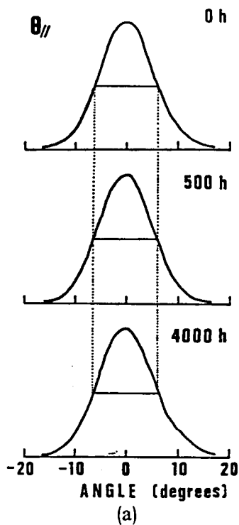
Fig.17 (a) A typical example of lateral far-field patterns measured before (0 h) and after the agings of 500 and 4000 h under 5 mW/facet at 50°C. (b) Relative change of full-width at half-power (FWHP) of far-field pattern from 0 h after aging.
