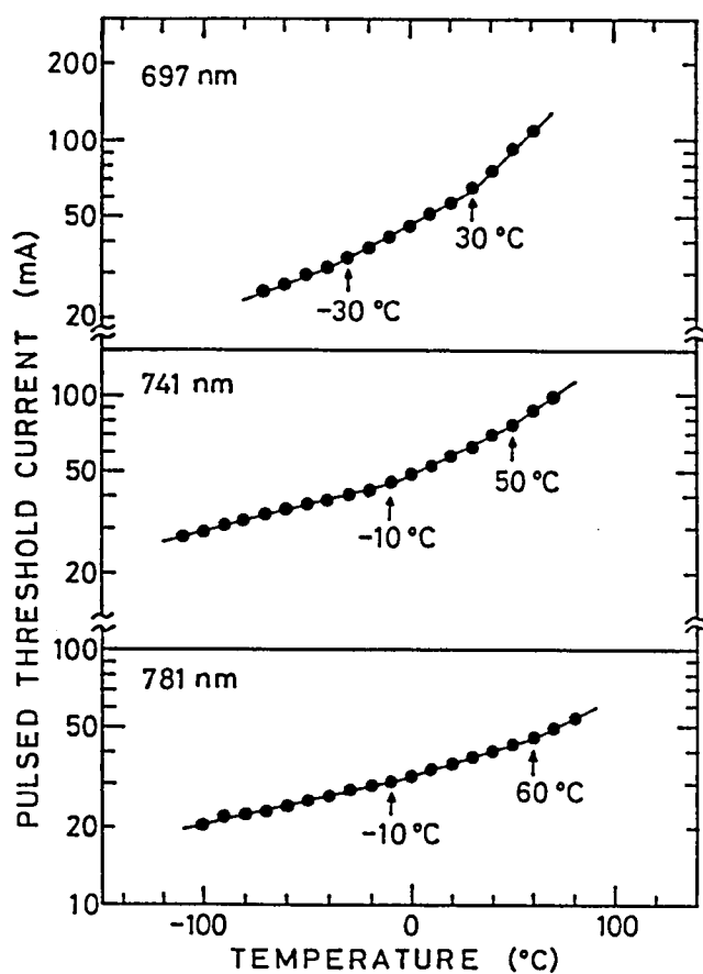
Fig.9 Temperature dependence of the threshold current of 697, 741, and 781 nm lasers.
