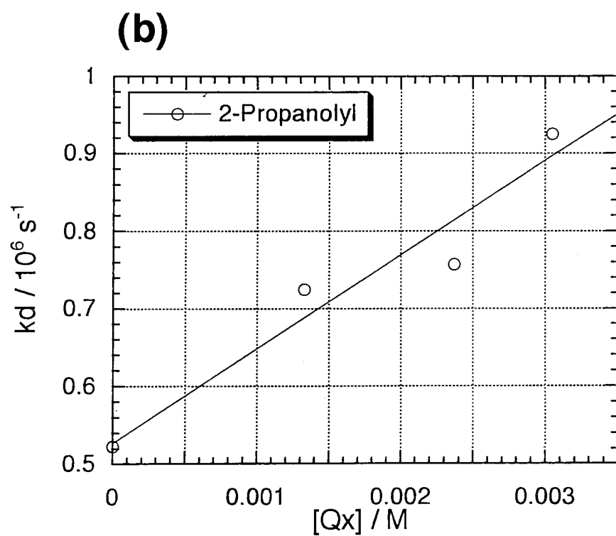
Figure 7-3 (a) The observed decay rate ( k_d = k_q[\text{Py}] + k_d^0 ) of 2-hydroxypropan-2-yl at 0^\circ\text{C} is plotted against the pyrazine concentration ( [\text{Py}] ). (b) A similar plot for the system of 0.01M pyrazine solution containing quinoxaline, temperature 0^\circ\text{C} .
