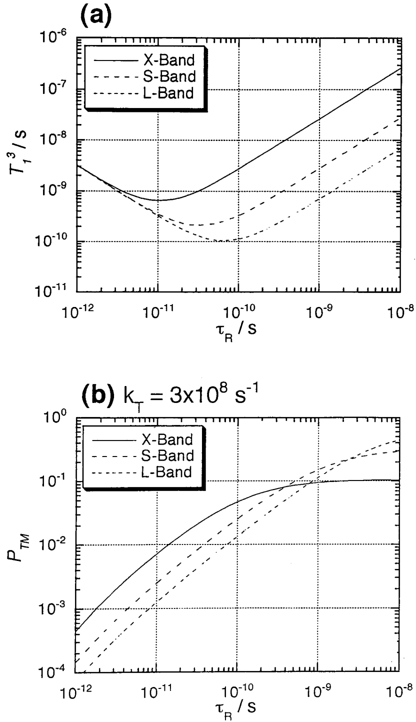
Figure 4-7 Calculated values of (a) ^3T_1 and (b) P_{TM} versus \tau_R in the X-, S-, and L-bands for the MA/ 2-propanol system obtained from eq.1 and 2. D = 3.0\text{GHz} , E = 1.0\text{GHz} , and k_T = 3 \times 10^8 \text{ s}^{-1} were used (see text).
