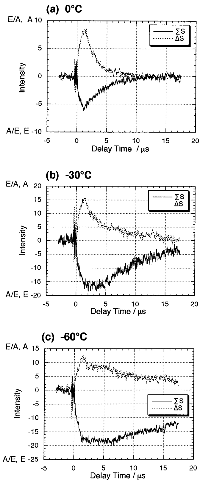
Figure 8-10 Time evolution of the net component ( \Sigma S ) and the antiphase component ( \Delta S ) of the transient EPR signal of the phenazine (0.0034M)/ 2-propanol system at (a) 0°C, (b) -30°C, and (c) -60°C.
