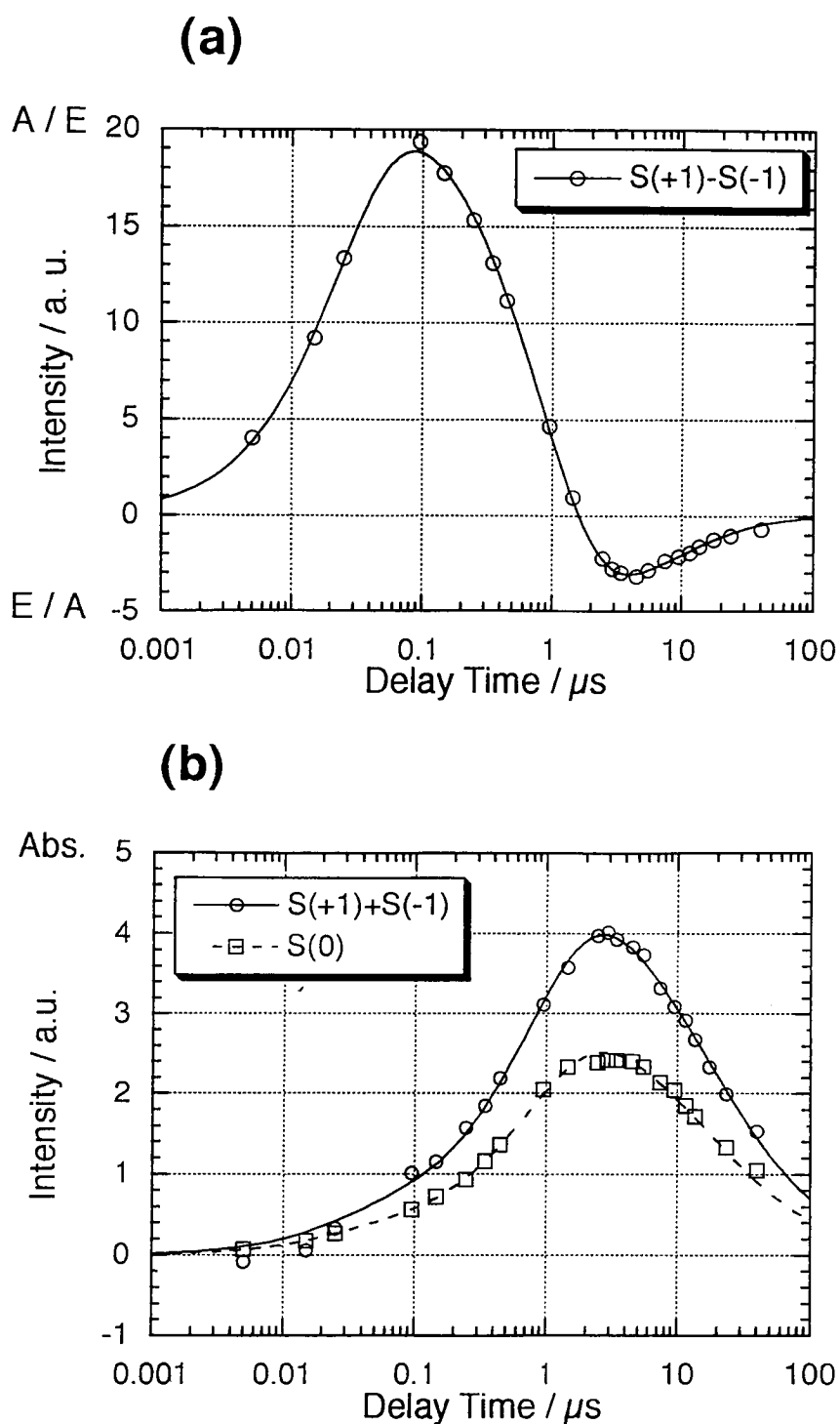
Figure 6-3. (a) The time evolution of \Delta S_M in the TEA solution. The solid line represents the result of a least-squares fit of the data points to eq.6-1.
