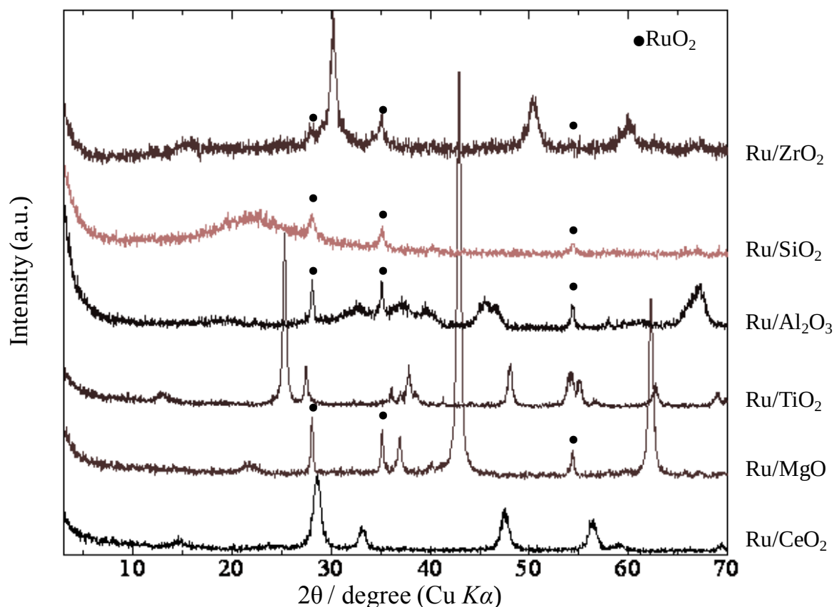
Figure 2. XRD patterns of Ru/supported catalysts.
