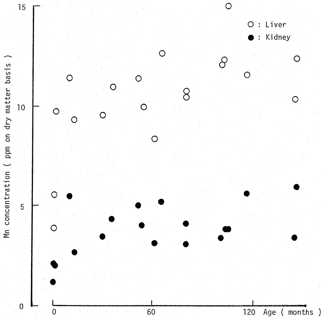
Fig. 4. Manganese concentration in liver and kidney of Holstein cattle kept at Kyushu Natl. Agric. Exp. Stn.
