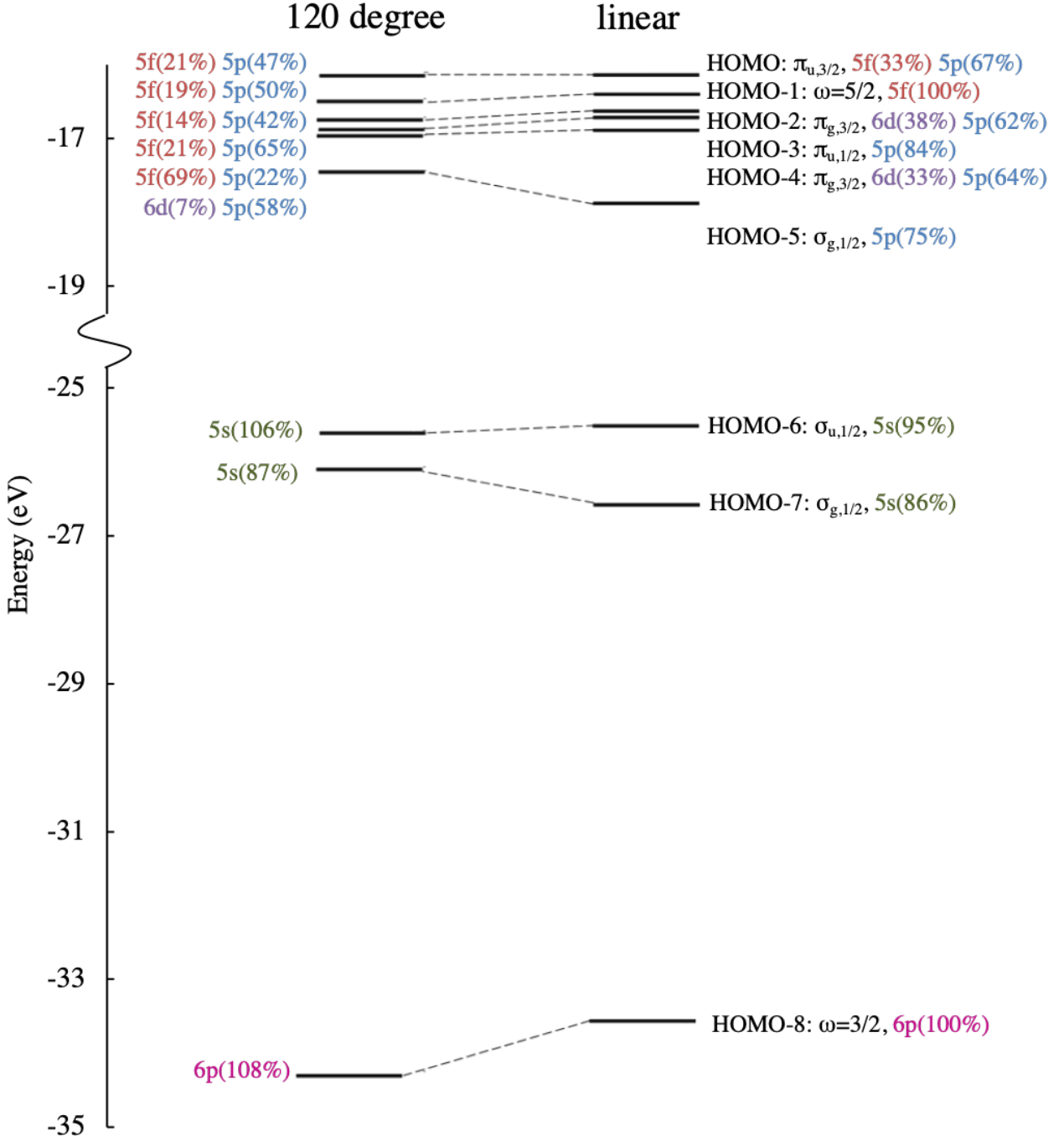
Figure 14: Walsh diagrams for \text{UTe}_2^{2+} ( R = 2.680 \text{ \AA} ) for the nine highest occupied orbitals. The dominant contributions of the atomic orbitals provided in Table S5 are also shown.
