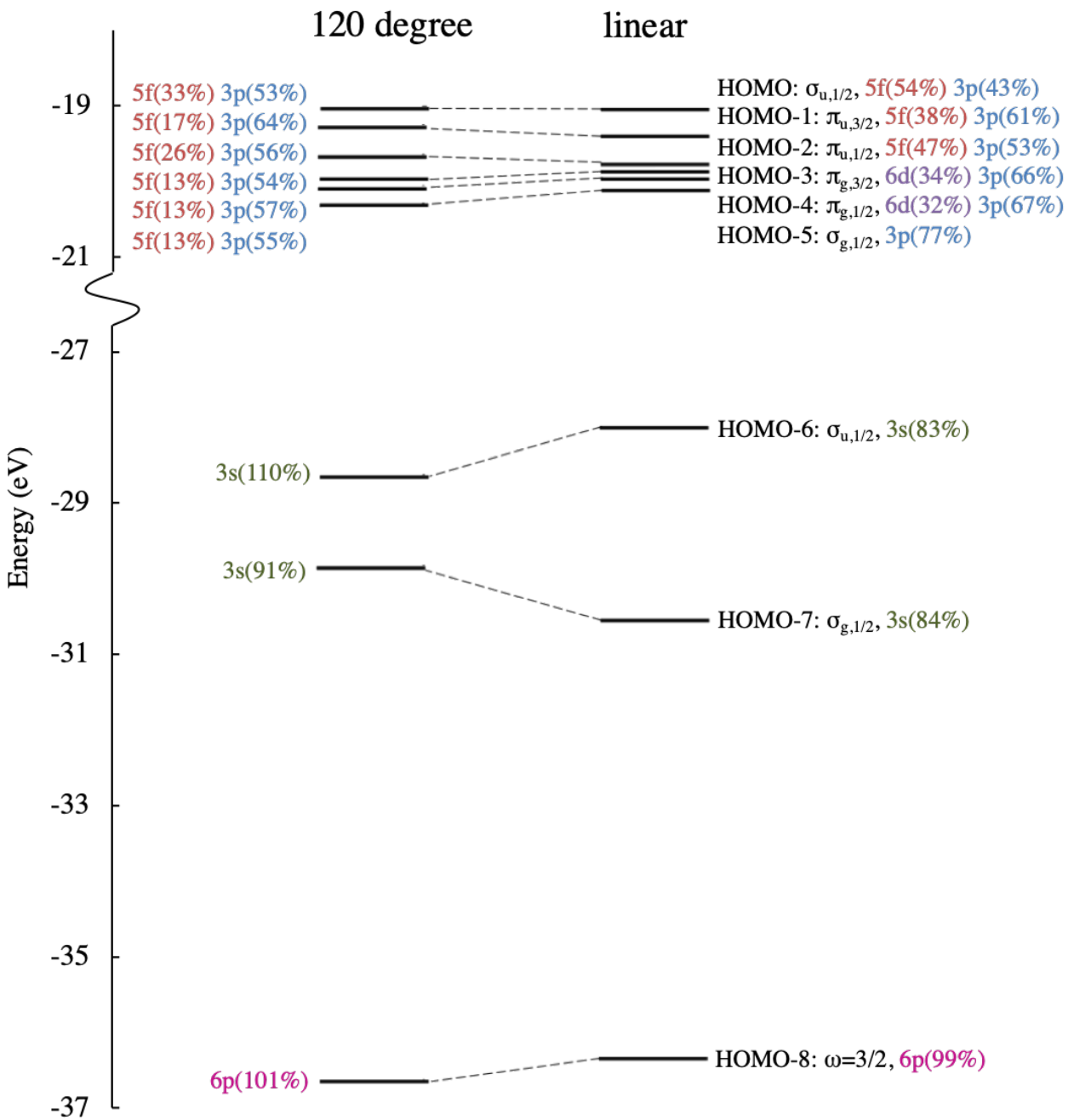
Figure 12: Walsh diagrams for \text{US}_2^{2+} ( R = 2.190 \text{ \AA} ) for the nine highest occupied orbitals. The dominant contributions of the atomic orbitals provided in Table S3 are also shown.
