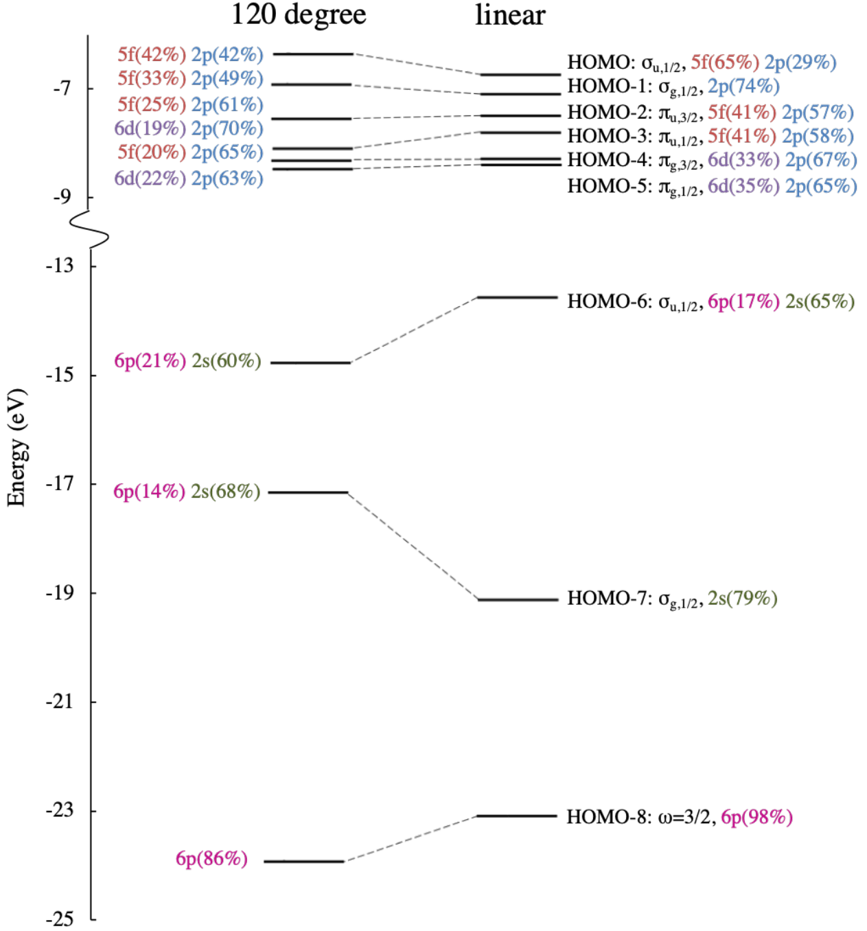
Figure 6: Walsh diagrams for \text{UN}_2 ( R = 1.736 \text{ \AA} ) for the nine highest occupied orbitals. The dominant contributions of the atomic orbitals provided in Table S2 are also shown.
