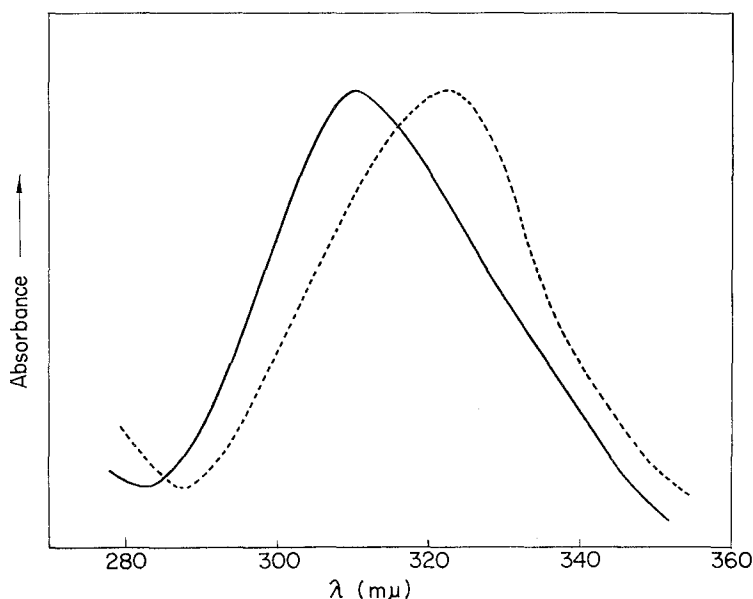
Fig. 4. Ultra-violet absorption spectra of neodymium benzoyltrifluoroacetate ( 2 \times 10^{-5} \text{M} ) in n -hexane containing 6 \times 10^{-5} \text{M} of ethyl alcohol, —; pyridine, — —; or n -butyl amine, ·····.
