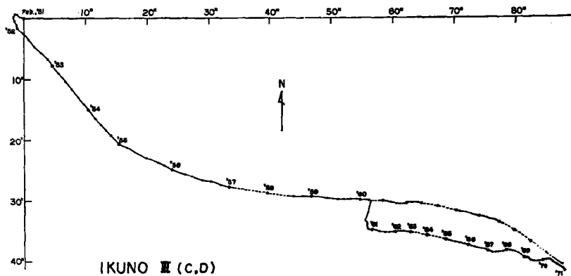
Fig. 7 Vector diagram of ground tilts observed at IKUNO III (C, D).
