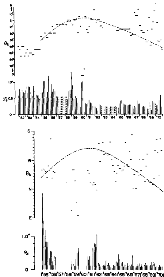
Fig. 8 Variation of direction ( \theta_t ) and change of total amount ( \phi_t ) of ground tilts per a month at Ikuno III.
