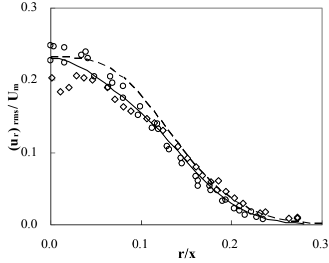
Fig. 3.3 Distribution of turbulent intensity of the radial velocity in a round jet without swirl
