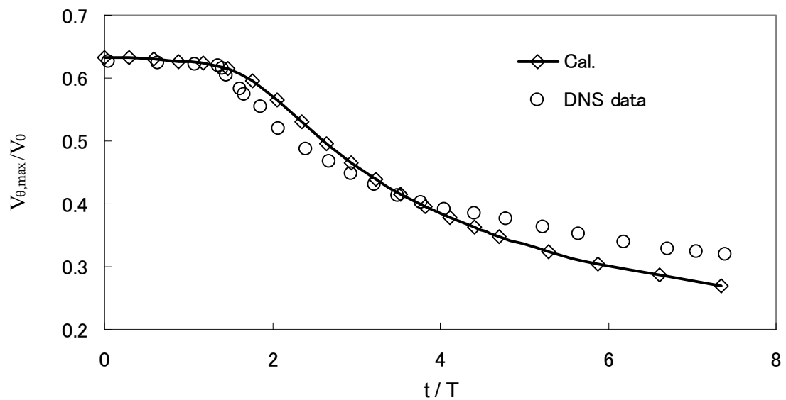
Fig. 6.25 Time decay of maximum tangential velocity (at r = r_0(t) ) compared with DNS results of Duraisamy and Lele (2006) for q = 0.5
