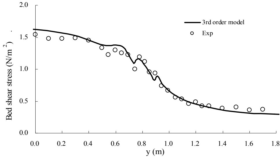
Fig. 5.17: calculated spatially averaged boundary shear stress profile for case C1 compared with the experimental results by Shiono and Knight (1991)
