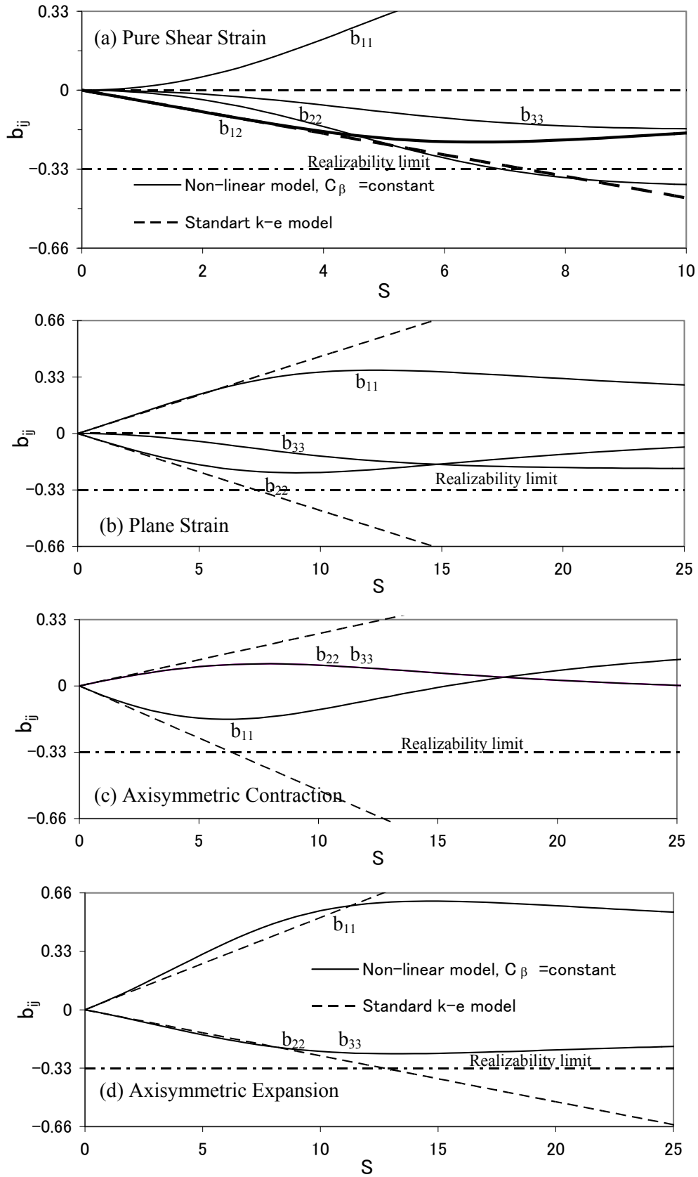
Fig. 2.6. The anisotropy of turbulence for the baseline flows in homogeneous strain predicted by (i) Non-linear k - \varepsilon model with c_\beta = \text{constant} and (ii) Standard k - \varepsilon model.
