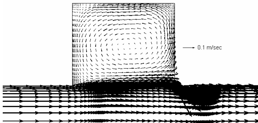
Fig. 7.4. Time averaged velocity vectors
