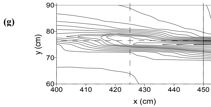
Fig. 5.21 Turbulent structures at the saddle point ( x = 400\text{--}450\text{ cm} ): (a) plan view of flow vectors (b) k (c) \varepsilon (d) \overline{u_1 u_1} (e) \overline{u_2 u_2} (f) \overline{u_3 u_3} (g) \overline{u_1 u_2}
