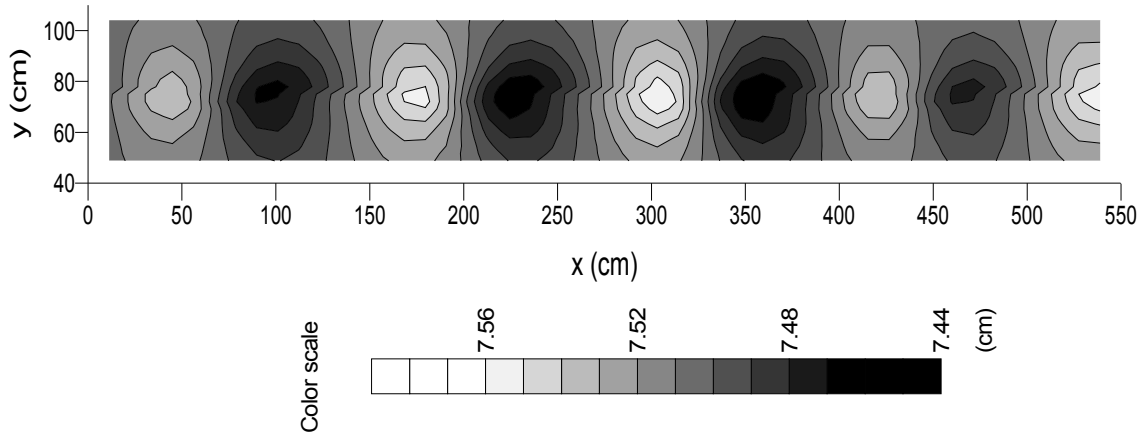
Fig. 5.5: Water surface distribution near the interface for the flow field shown in Fig. 5.4 (b)
