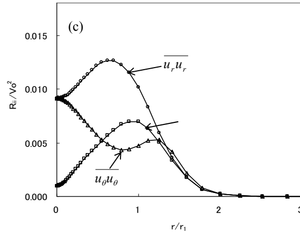
Fig. 6.17 Radial distribution of turbulent intensities at three directions at (a) t=3.72 T
