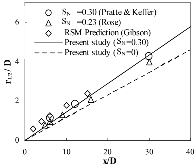
Fig. 3.8 Comparison of jet half-width
