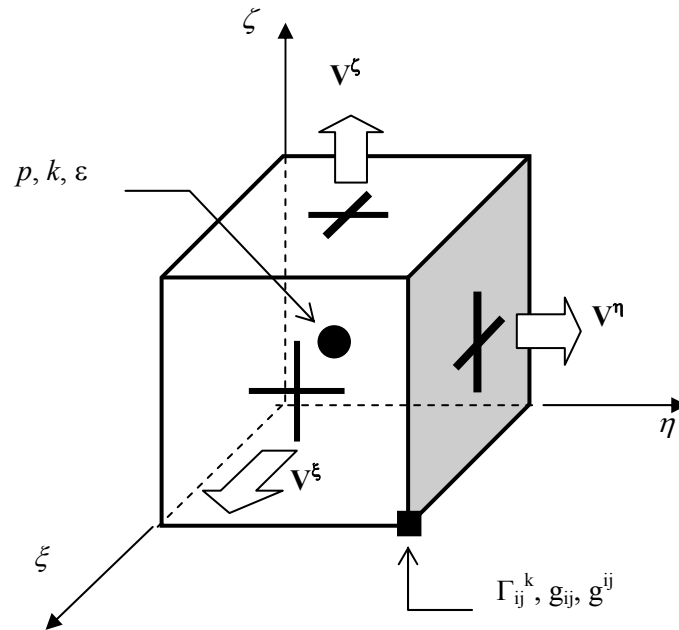
Fig. 7.2 Arrangements of variables in a staggered grid in the 3D computations (Curvilinear coordinate system)
