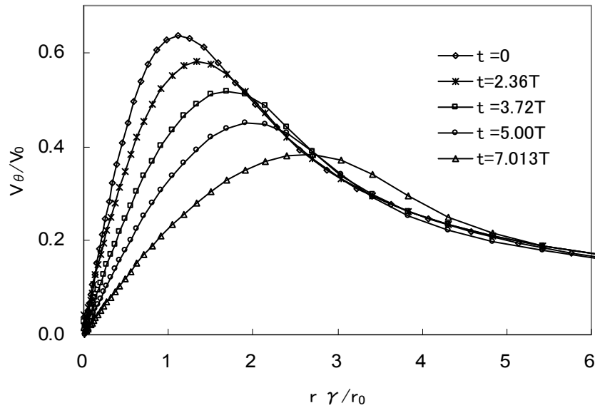
Fig. 6.6 Radial distribution of tangential velocity and its decay with time (Non-linear k-\varepsilon model)
