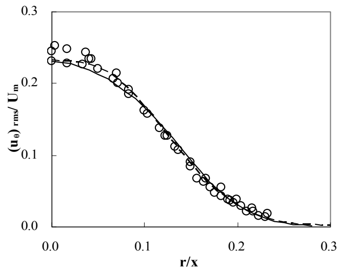
Fig. 3.4 Distribution of turbulent intensity of the circumferential velocity in a round jet without swirl
