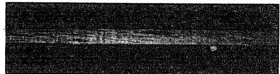
Photo. 3 Typical patterns of breaking in the radial test of Buna. The fracture propagated from left to right.
