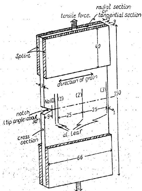
Fig. 4. Form and size of our specimen.
