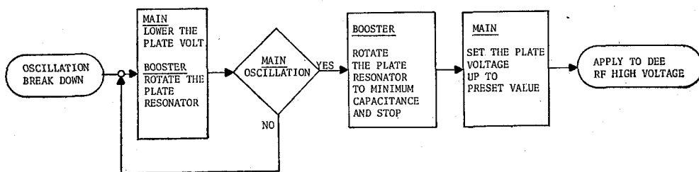
Fig. 6-6. Control system of the oscillator. Automatic recovery method of the oscillation is also shown.
