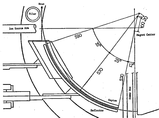
Fig. 5-11. Dimensions of the deflector.
