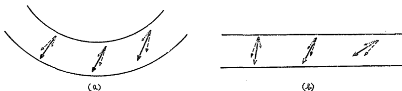
Fig. 32. Configuration of remanent magnetization of Sasayama red bed in relation to the bending of stratum. — J_r : natural remanent magnetization, ..... J_r' : magnetic moment disappeared at 330^\circ\text{C} (magnetization due to \text{FeS}_{1+x} ), ——— J_r'' : remanent magnetic moment at 330^\circ\text{C} (magnetization due to \text{Fe}_3\text{O}_4 and \alpha\text{-Fe}_2\text{O}_3 ). (a) Direction of remanent magnetization of the bed, whose local dip is not corrected, (b) Direction of remanent magnetization of the bed, whose local dip is corrected.
