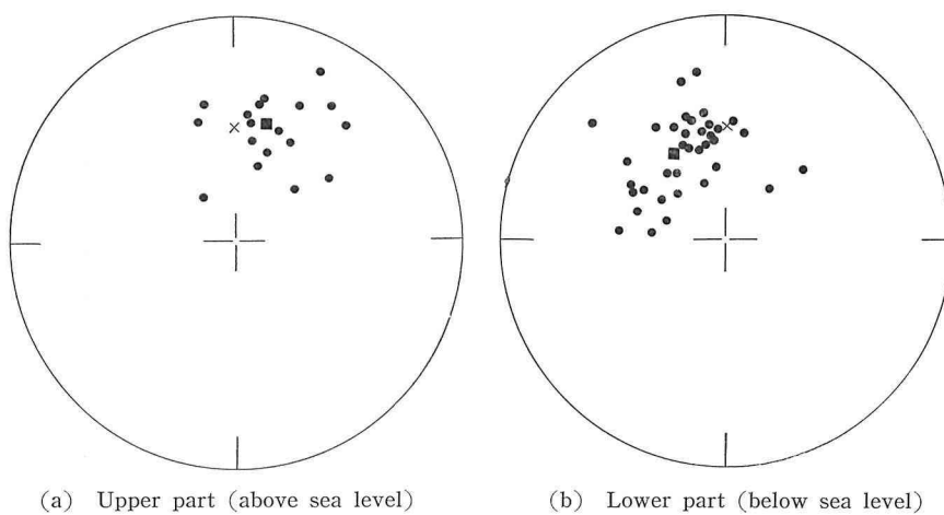
Fig. 4. Direction of the natural remanent magnetization of upper part and lower part of the ore-deposit. \times : Direction of the present dipole field, \blacksquare : Mean direction of the n.r.m..
