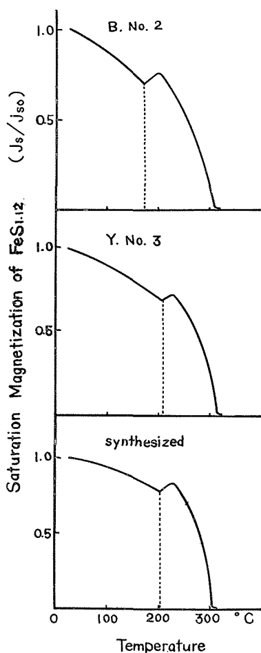
Fig. 22. Characteristic difference in thermo-magnetic curves of Besshi, Yanahara and the synthesized \text{FeS}_{1.12} .
