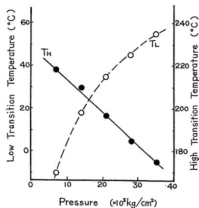
Fig. 18. Relationship between the transition temperature of \text{FeS}_{1.12} and the magnitude of the applied pressure. T_H represents the high temperature transition and T_L the low temperature transition.
