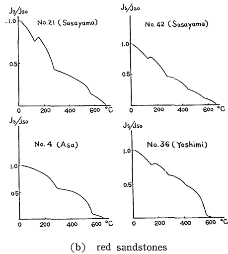
Fig. 25. Representative examples of the thermo-magnetic curves of black shales and red sandstones.
