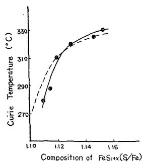
Fig. 13. Relationship between Curie temperature and the chemical composition of synthesized \text{FeS}_{1+x} . Dotted line shows the result obtained by Haraldsen (1937).
