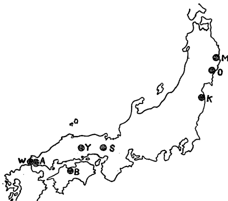
Fig. 1. Distribution of the collecting sites. Samples of iron-sulfide ore-deposits were collected from the places B and Y, red sandstones from S, A and W, and black shales from W, M, O and K.
