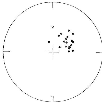
Fig. 8. Direction of the n.r.m. of Yanahara ore-deposit.
