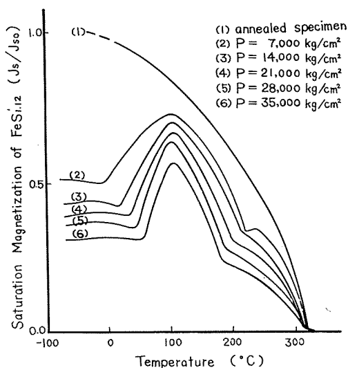
Fig. 17. Change of the intensity of the saturation magnetization of \text{FeS}_{1.12} observed in a thermo-magnetic analyses after the application of one-directional pressures.
