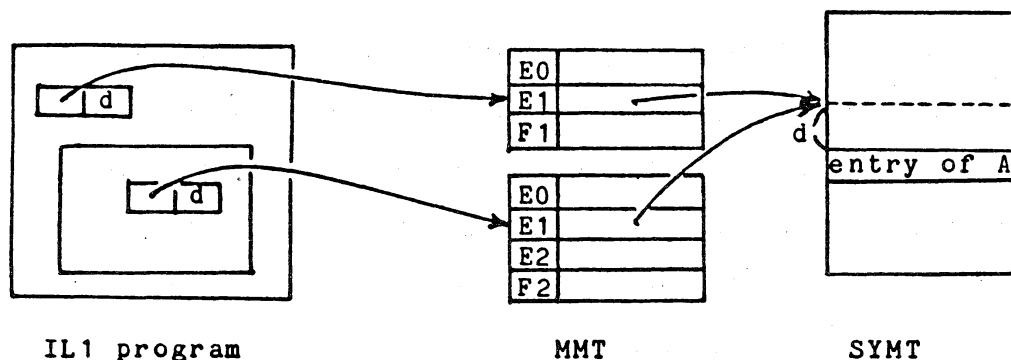
(c) The internal structure of the expanded program.
