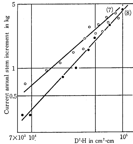
Fig. 3. Allometric relation dry weight of current annual stem increment ( \Delta w_s ) in kg and D^2H in \text{cm}^2\text{cm} .
