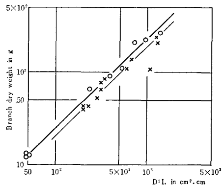
Fig. 10. Relation between oven dry weight and volume showing cross-sectional area of base ( D^2 ) \times length ( L ) of branches. ○ : Upper layer branches × : Under layer branches
