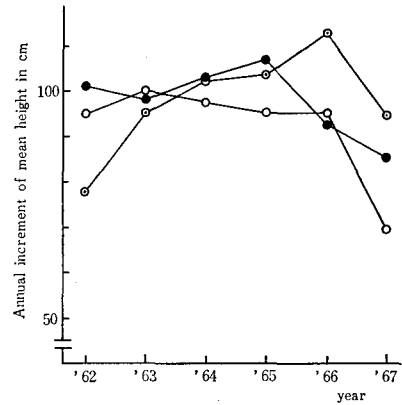
Fig. 4. Annual increment of mean tree height in each year.
