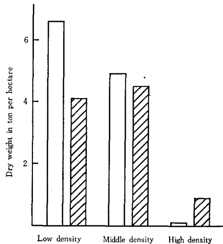
Fig. 14. Oven dry weight of ground flora in each stand.
