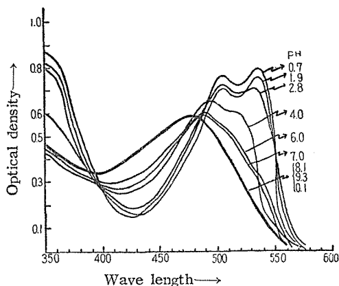
Fig. 2. Absorption spectra of 1.5 \times 10^{-4} M of the reagent at various pH's.
