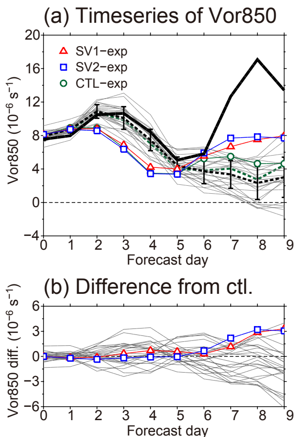
Fig. 5. (a) Daily time series of 850-hPa relative vorticity (unit: 10^{-6} \text{ s}^{-1} ) averaged over the verification area [ 15^{\circ}\text{--}30^{\circ}\text{N} , 125^{\circ}\text{--}150^{\circ}\text{E} ] in the re-analysis (black line), control run (green dashed line), all ensemble members (gray thin line), and the ensemble mean (black dashed line) from the initial time to the lead time of +9 day (25 August 2016). Error bars denote the ensemble spread represented by 1 standard deviation. Red triangles, blue squares, and green circles connected by lines indicate the results of the SV1-, SV2-, and CTL-experiments, respectively. (b) Same as (a) but the differences from the control run for the ensemble members (gray thin line) and those from the CTL-experiment for the SV1-experiment (red line) and SV2-experiment (blue line), respectively.
