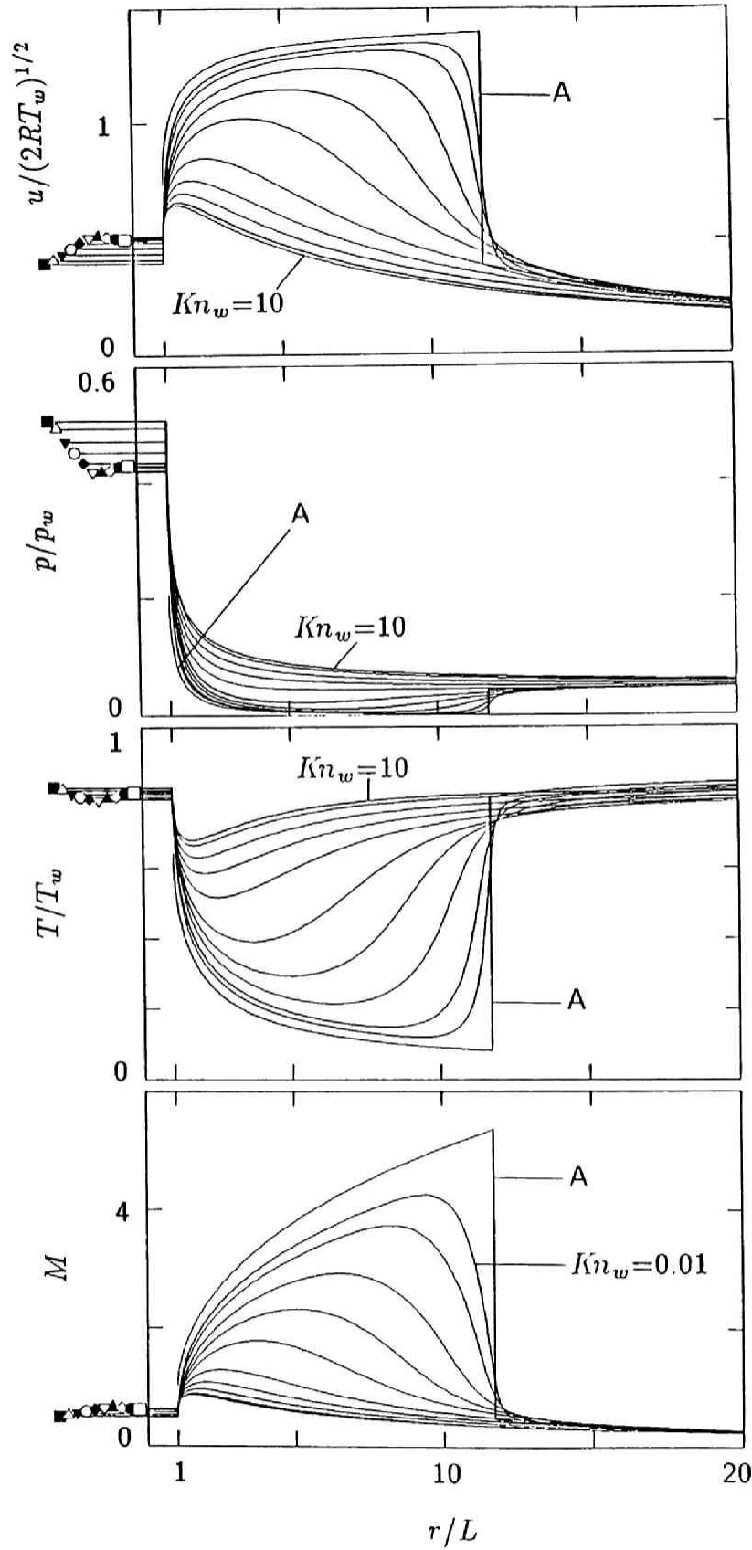
Fig. 3-14. The distributions of the nondimensional macroscopic variables, the flow velocity u/(2RT_w)^{1/2} , the pressure p/p_w , the temperature T/T_w , and the Mach number M(= u/(5RT/3)^{1/2}) , for various Knudsen numbers Kn_w VI: Case p_\infty/p_w = 0.05 . (See the caption of Fig. 3-9.)
