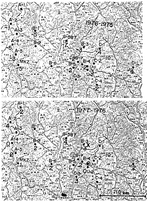
Fig. 6. Secular changes of geomagnetic total force relative to Tottori.
