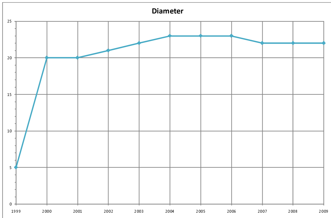
Figure 3.18: The Diameter of SourceForge.net Network Over Time
