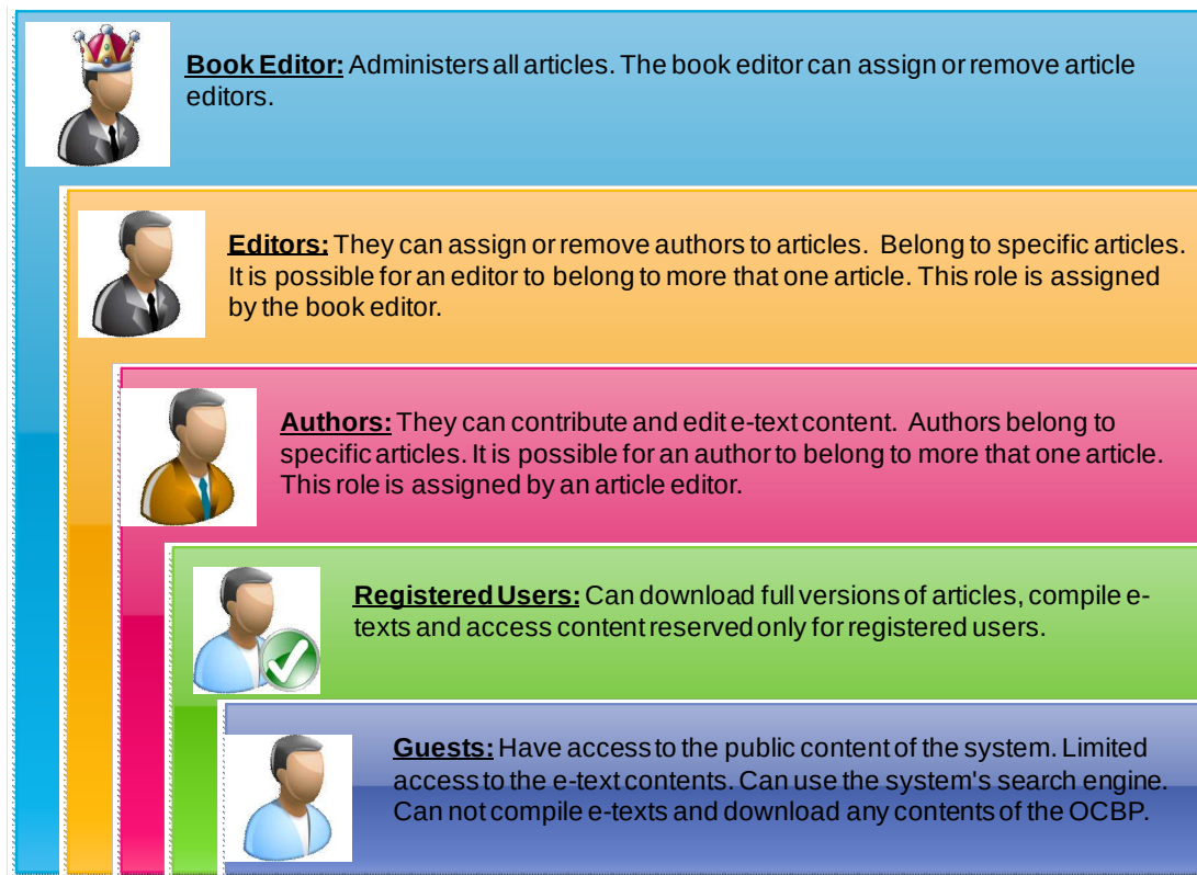
Figure 6.5: The OCBP Access Layer
