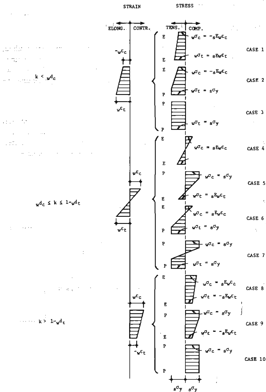
Fig. 7. Ultimate State of Steel Web.
