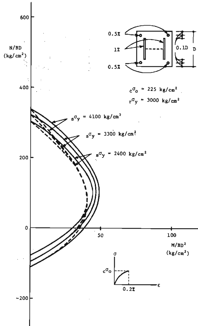
Fig. 18. Effects of Stress-Strain Relationship of Concrete—(IV).
