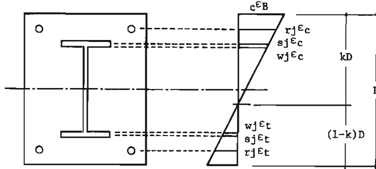
Fig. 5. Strain Distribution.
