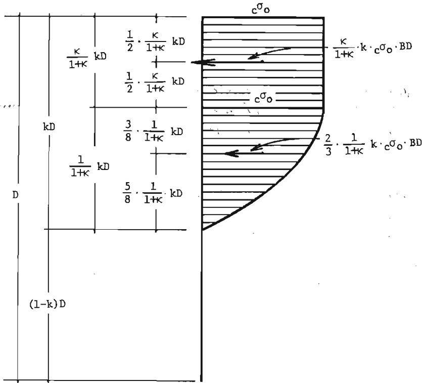
Fig. 4. Stress in Concrete at Ultimate State.
