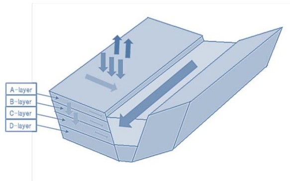
Fig.3 Schematic view of Hydro-BEAM
